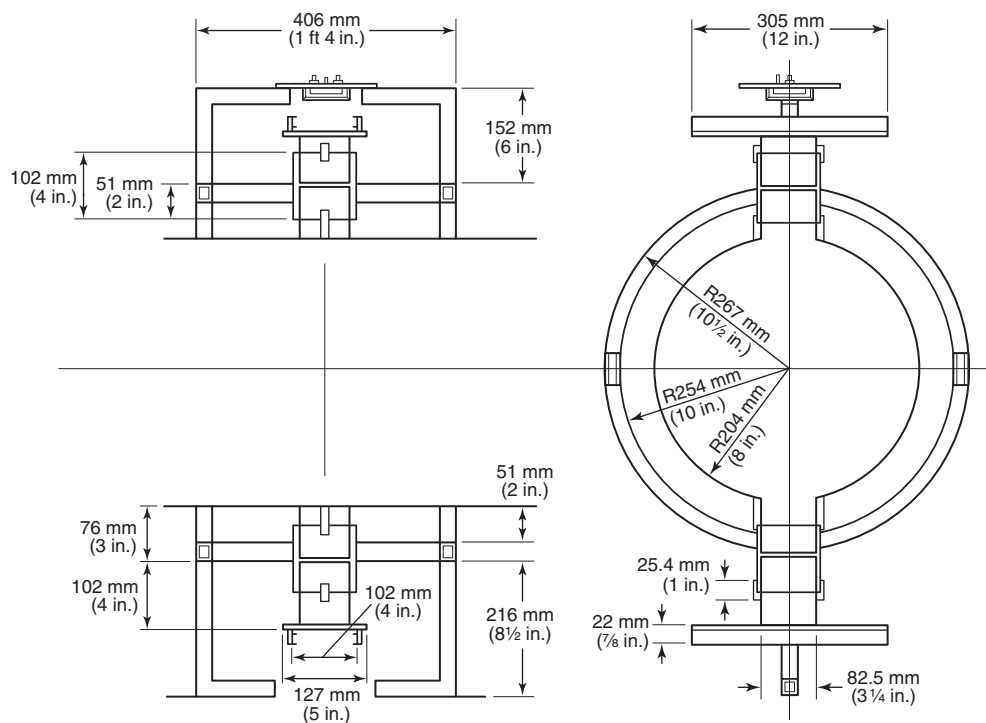
FIGURE C.2(n) Ring and Filter Holder Assembly Cross-Section.
