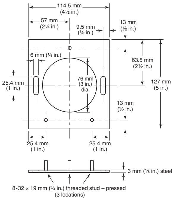
FIGURE C.2(j) Photocell Duct Cross Adjustment Plate.
