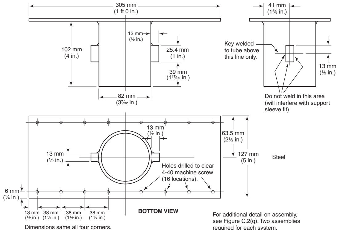
FIGURE C.2(f) Filter Holder Adapter Assembly.
