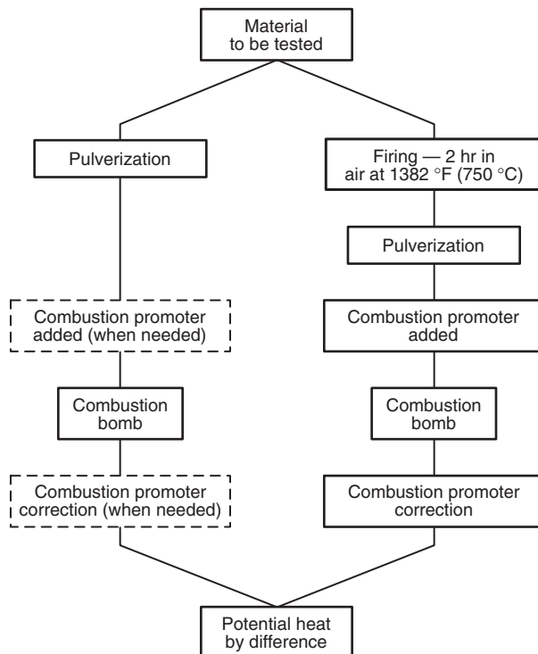
Figure 1-4 Schematic diagram of test procedure for potential heat measurements.
