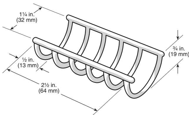
Figure 2-2.4 Wire specimen holder for muffle furnace firing.
