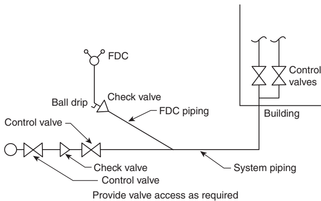
FIGURE A.5.9.3.2.1(b) Fire Department Connection Connected to Underground Piping (Sample 2).
