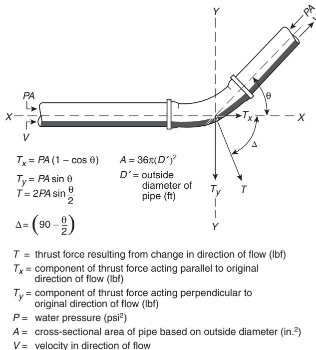
FIGURE A.10.6.1(a) Thrust Forces Acting on Bend.
