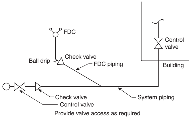
FIGURE A.5.9.3.2.1(a) Fire Department Connection Connected to Underground Piping (Sample 1).
