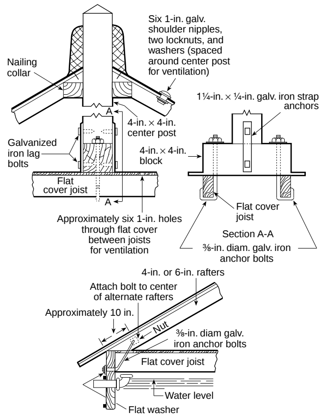
Figure B-3 Details of tank roof construction.
