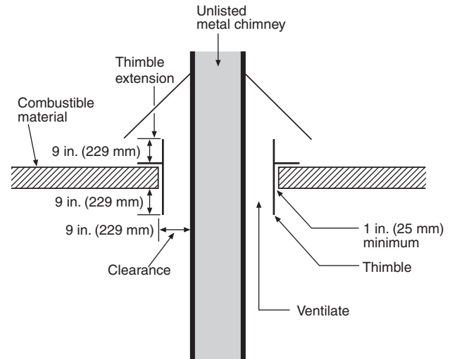
FIGURE 8.2.2.2.7 Ventilating Thimble.
