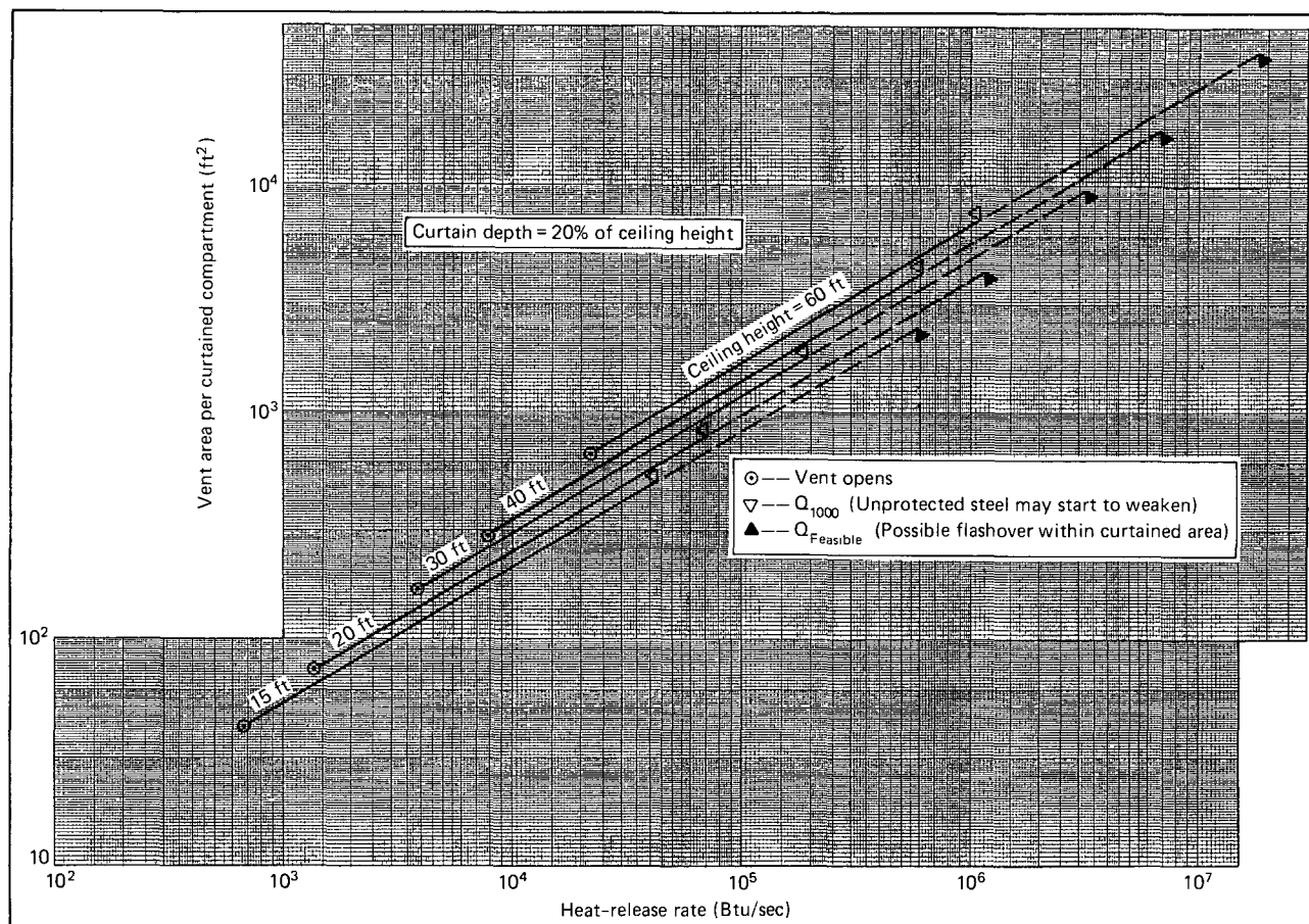
Figure 4-1 Limited Fire Growth: Recommended Vent Areas per Curtained Compartment for Various Maximum Heat-Release Rates (Btu/second).
