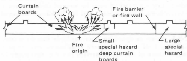
Figure 1-1 Behavior of Combustion Products Under Vented and Curtained Roof.
