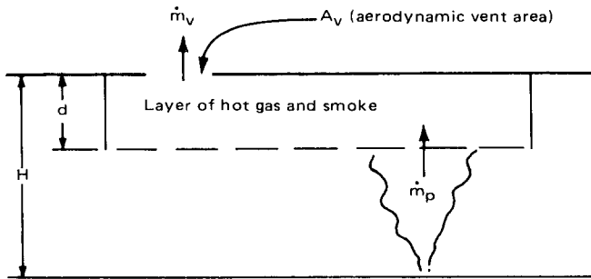
Figure A-1 Schematic of Venting System.
