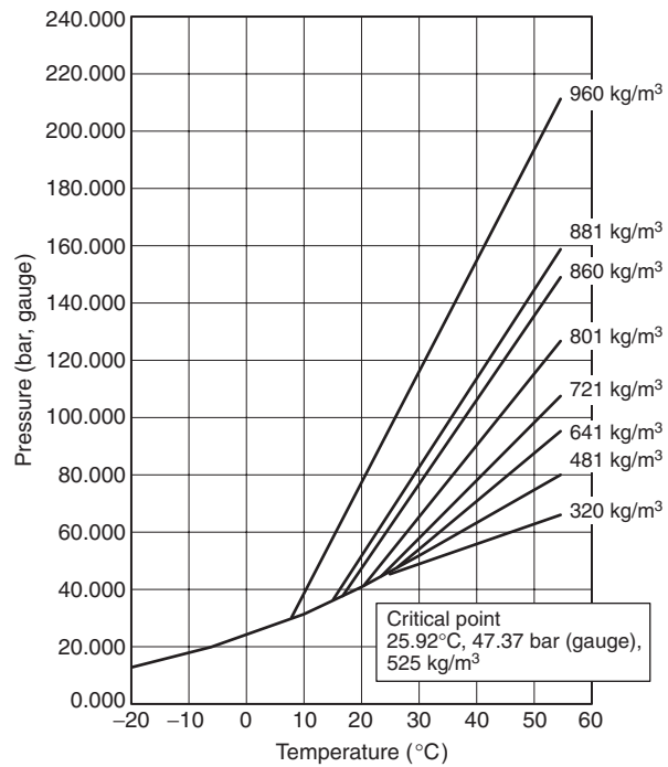
FIGURE A.4.1.4.1(g) Isometric Diagram of HFC-23.
