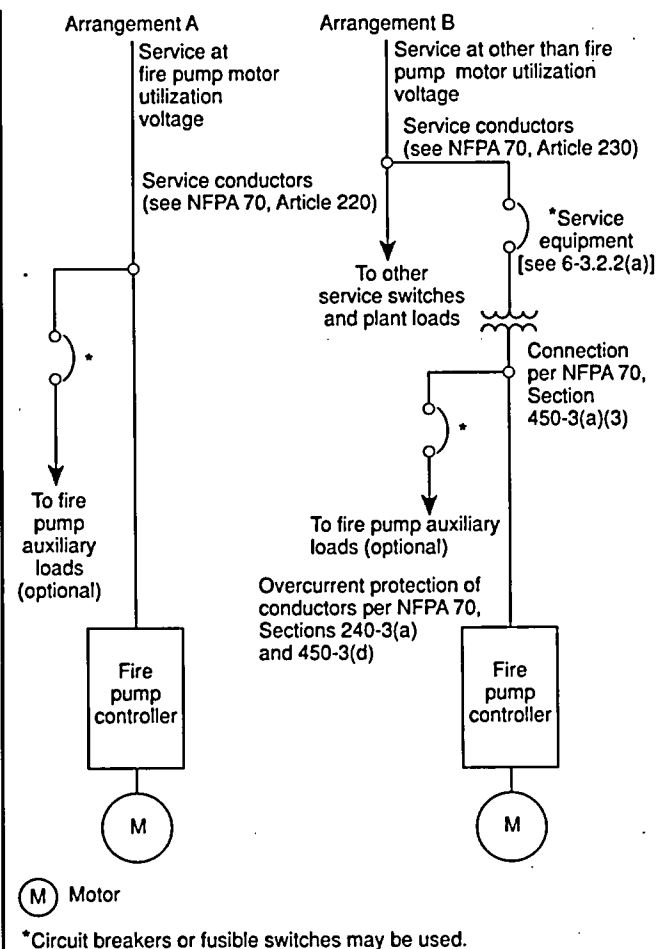
Figure A-6-3.2 Typical power supply arrangements from source to motor.
