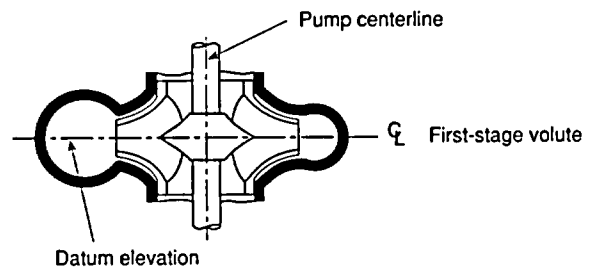
(2) Vertical double-suction pump
