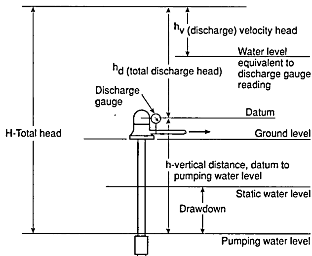
Figure A-1-7(c) Total head of vertical turbine-type fire pumps.
