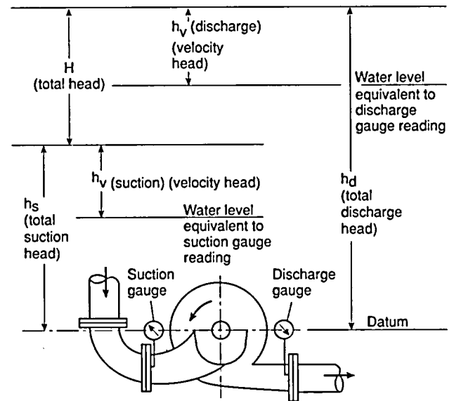
Installation with suction head above atmospheric pressure shown
