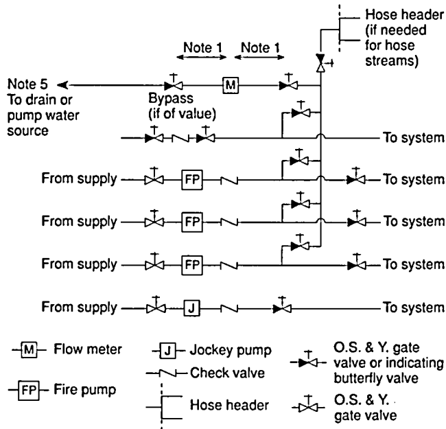
Figure A-2-14.1.2(a) Diagram of preferred arrangement for measuring fire pump water flow with meter for multiple pumps and water supplies, water discharge to drain or to pump water source.
