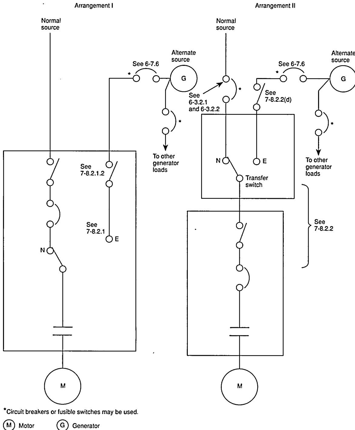
Figure A-7-8 Typical fire pump controller and transfer switch arrangements.
