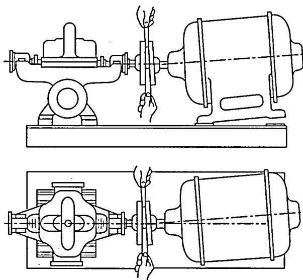
Figure A-3-5(a) Checking angular alignment. 1
