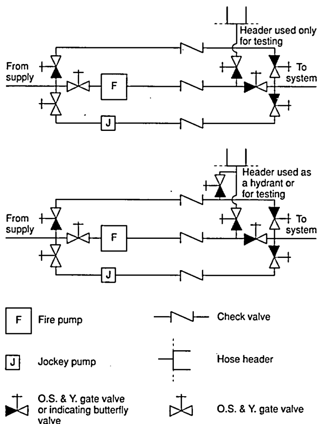
Figure A-2-9.5 Schematic diagram of suggested arrangements for a fire pump with a bypass, taking suction from public mains.
