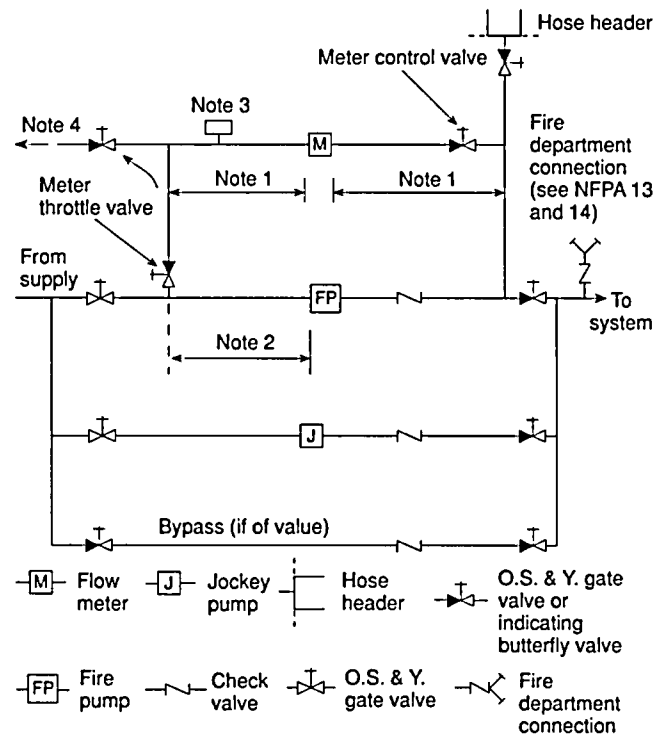
Figure A-2-14.1.2(b) Diagram of typical arrangement for measuring fire pump water flow with meter, discharge to pump suction.
