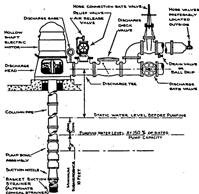
Figure A-4-2.1 Vertical Shaft Turbine-type Pump Installation in a Well.
