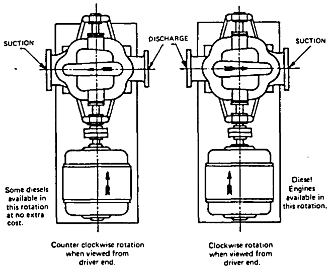
Figure A-2-16(b) Horizontal Pump Shaft Rotation.
