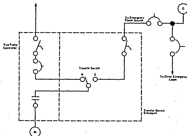
Figure A-7-8.3 One Method of Automatic Transfer Switch Installation for Two Power Sources.
