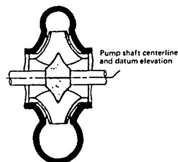
Horizontal Double Suction Pump
