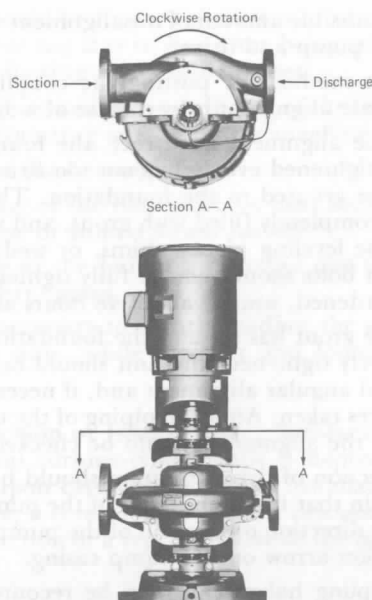
Figure A-2-16(c) Vertical Pump Shaft Rotation.
