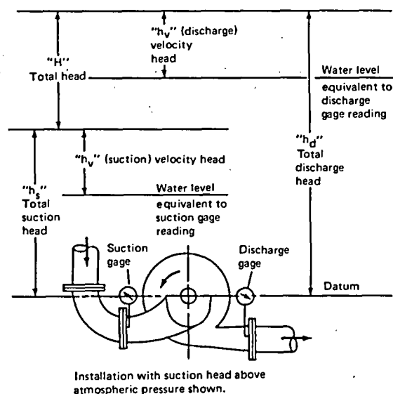
Figure A-1-7.5.7 Total Head of all Types of Centrifugal (Not Vertical Turbine-type) Fire Pumps. Pictorial does not show the various types of pumps applicable.
