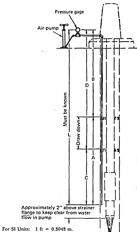
Figure A-4-3.5.3 Air Line Method of Determining Depth of Water Level.
