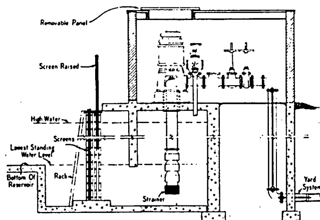
Figure A-4-2.2 Vertical Shaft Turbine-type Pump — Installation in a Wet Pit.
