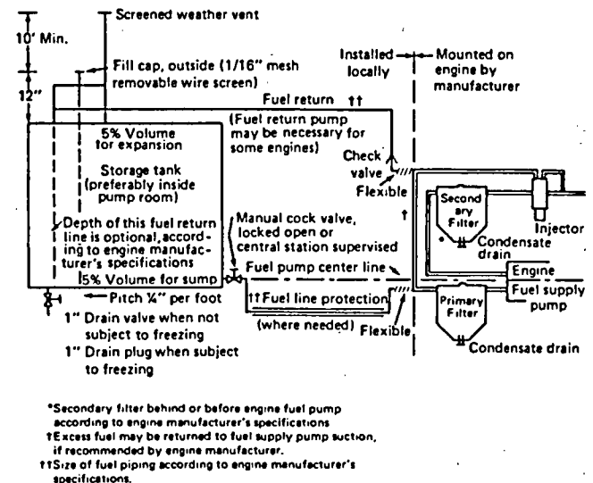
Figure A-8-4.6 Fuel System for Diesel Engine Driven Fire Pump.
