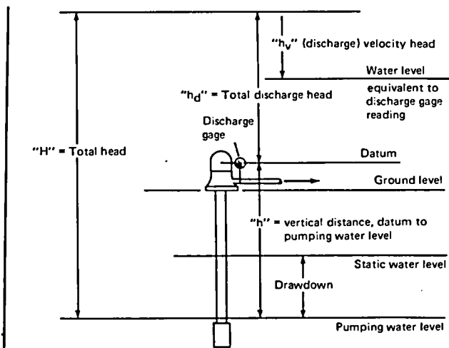
Figure A-1-7.5.8 Total Head of Vertical Turbine-type Fire Pumps.
