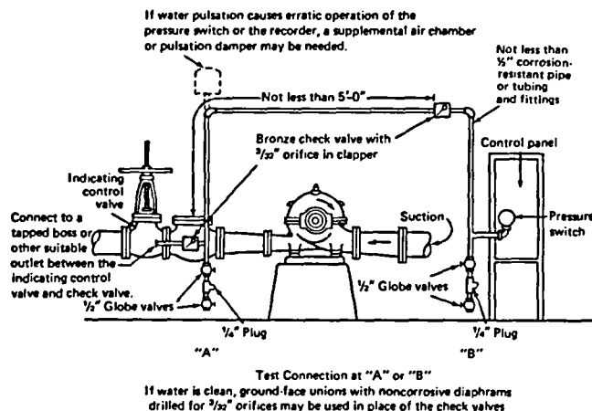
Figure A-7-5.2.1 Piping Connection for Each Automatic Pressure Switch (for Fire Pumps or Jockey Pumps).
