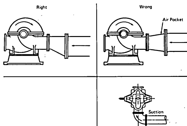
Figure A-2-9.6 Right and Wrong Pump Suctions.
