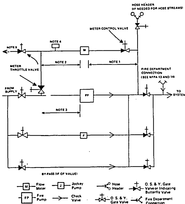
Figure A-2-13.2.1(b) Diagram of Typical Arrangement for Measuring Fire Pump Water Flow with Meter, Discharge to Pump Suction.
