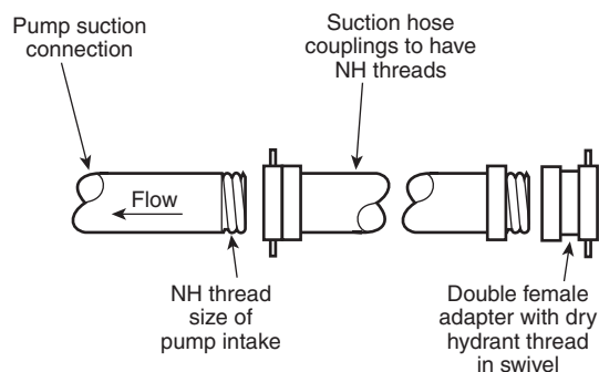
FIGURE A.4.4.6 Intake Connections from Dry Hydrant to Pump.
