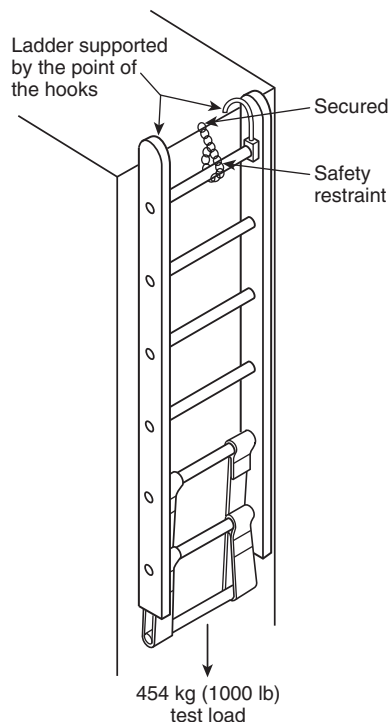
FIGURE 7.2.2.2 Roof Ladder Positioned for Roof Hook Test.
