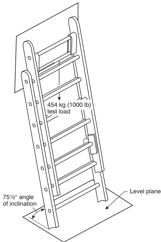
FIGURE 7.2.3.2 Extension Ladder Positioned for Hardware Test.
