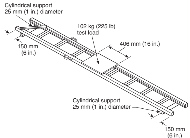
FIGURE 7.4.1 Folding Ladder Positioned for Horizontal Bending Test.
