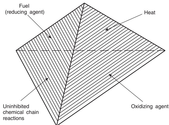
FIGURE 5.5 Fire Tetrahedron ([921:5.1.5]).
