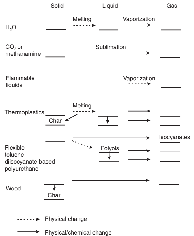
FIGURE 5.6.2 Phase Changes.
