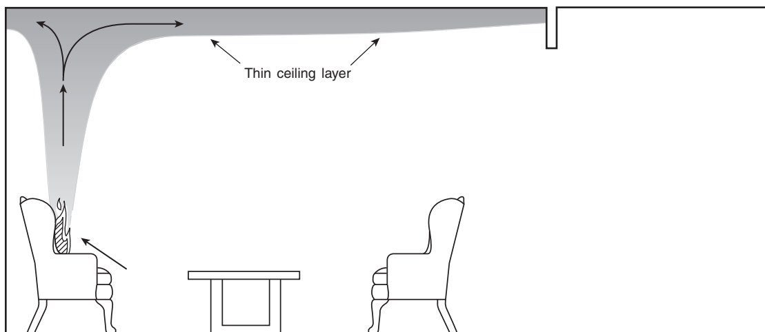
FIGURE 6.4.2.1.1.4 Early Compartment Fire Development.
