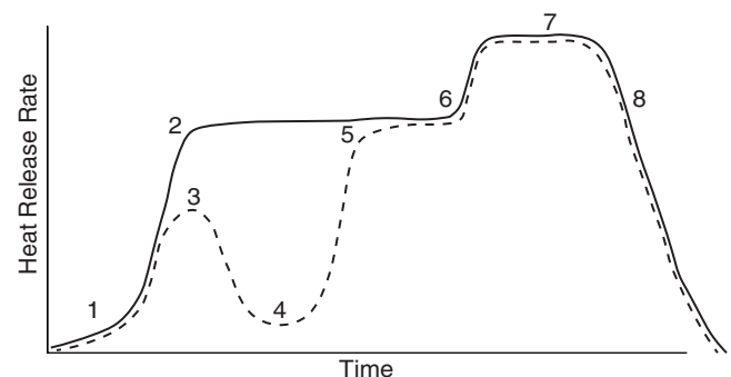
FIGURE 6.4.2 Fire Progression in Ventilated Versus Unventilated Compartments.
