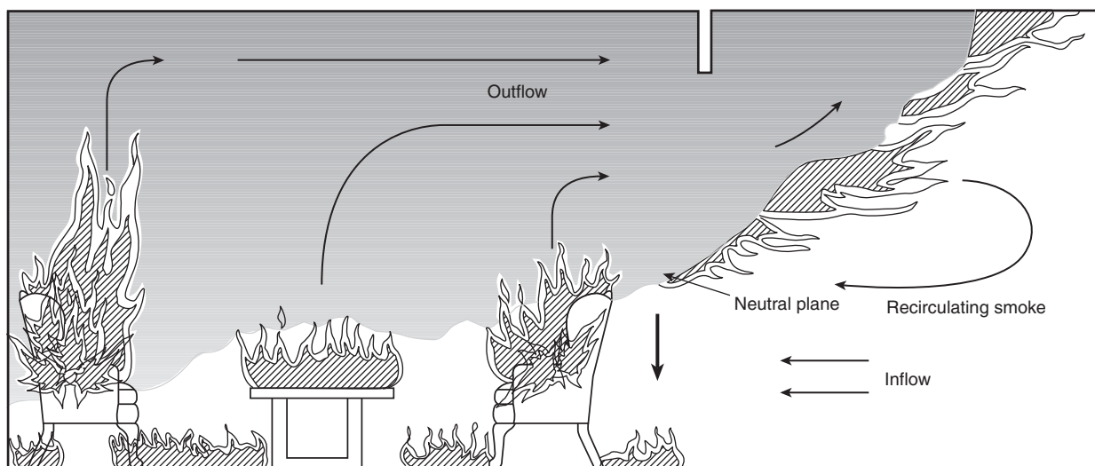
FIGURE 6.4.2.1.2 Flashover Conditions in Compartment Fire.
