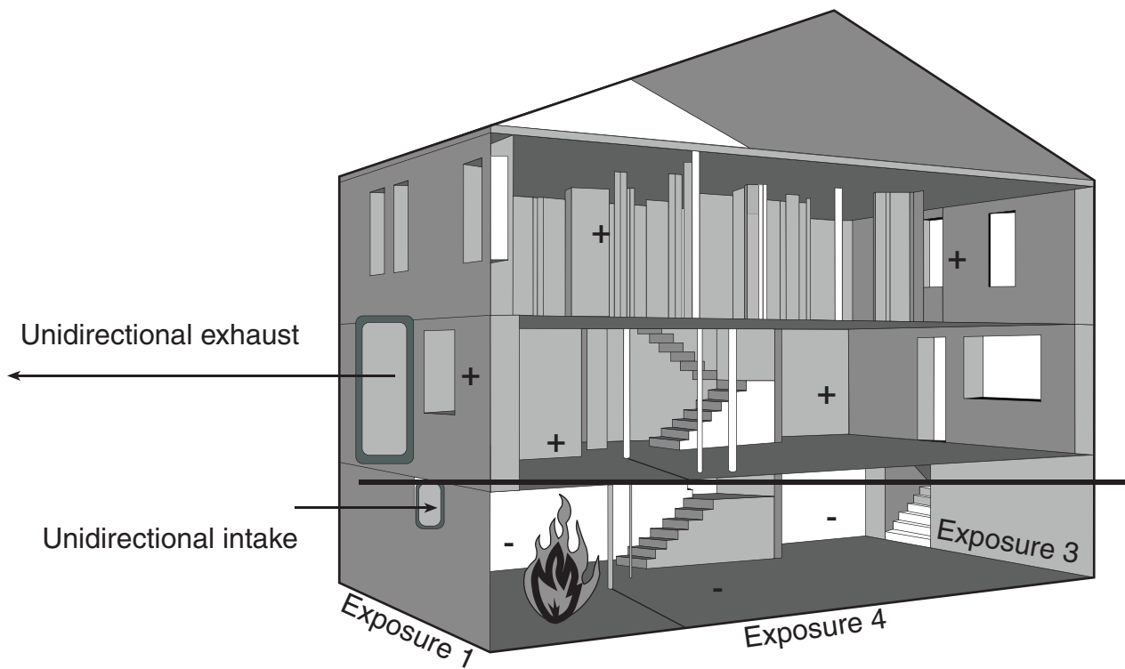
FIGURE 6.5.9 Unidirectional Flow Path.
