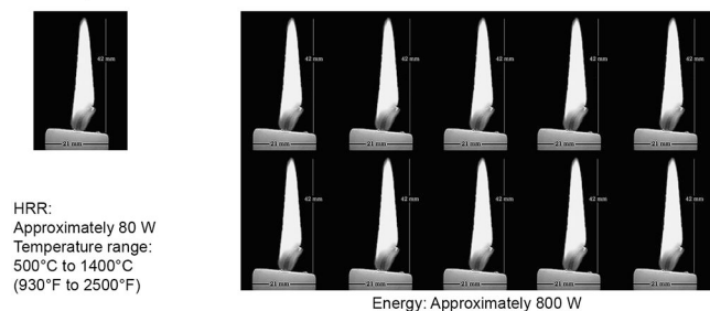
FIGURE 5.5.3.3 Heat Release Rate Versus Temperature Visualization.
