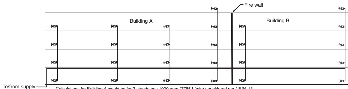
FIGURE A.7.10.1.2.3.1 Common Supply Piping Standpipes Calculated.
