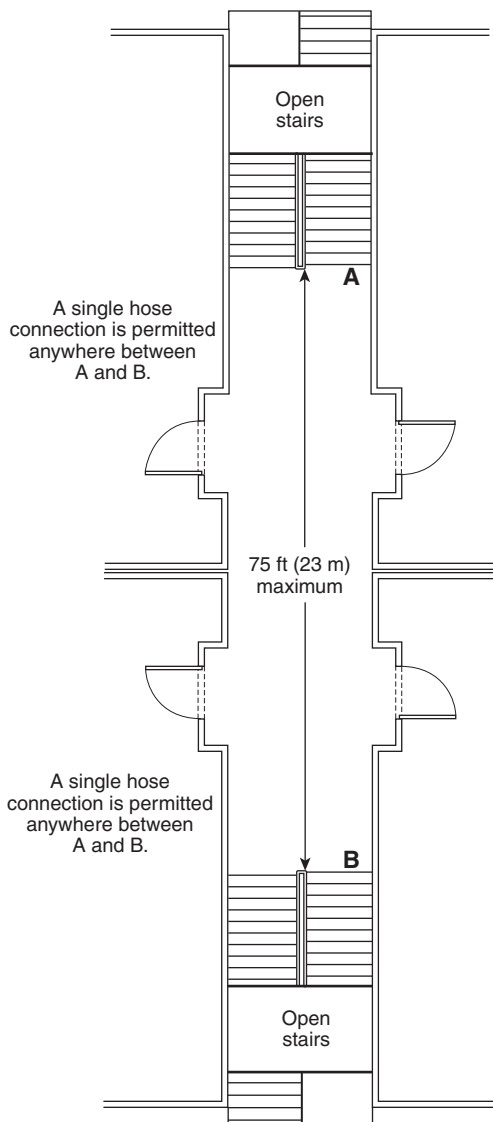
▲ FIGURE A.7.3.2.5 Single Hose Valve in Open Stairs/Corridors.
