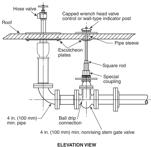
FIGURE A.7.3.2.7 Roof Hose Connection Piping Arrangement.
