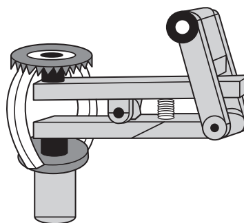
FIGURE 5.2.1 Sprinkler with Sprinkler Wedge Installed.
