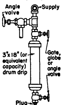
Fig. 3230. Auxiliary Drains.
