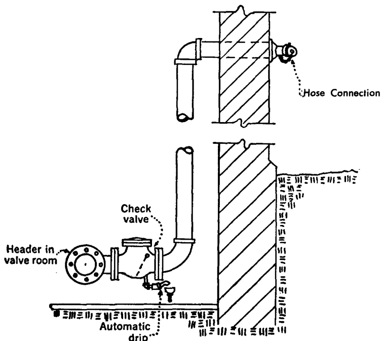
Fig. 2600. Fire Department Connection.
