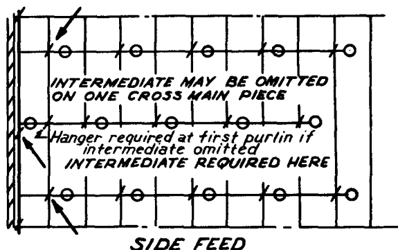
Fig. 3573. Hanger Omissions on Side Feed System.
