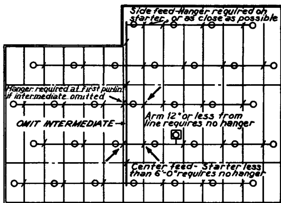
Fig. 3567. Hanger Omissions.
