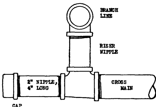
Fig. 3064. Flushing Connection.
