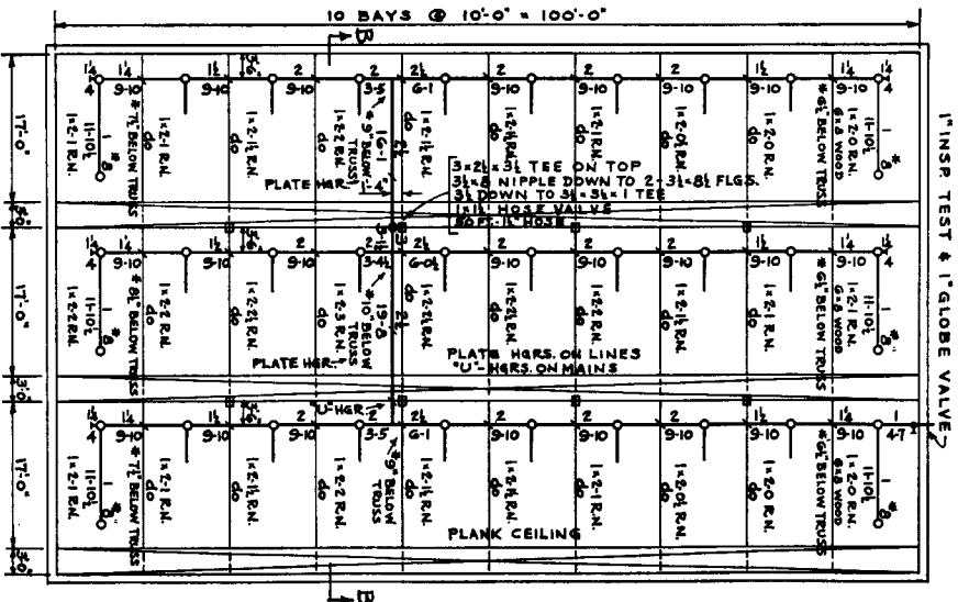
SECOND FLOOR OR ROOF PLAN
