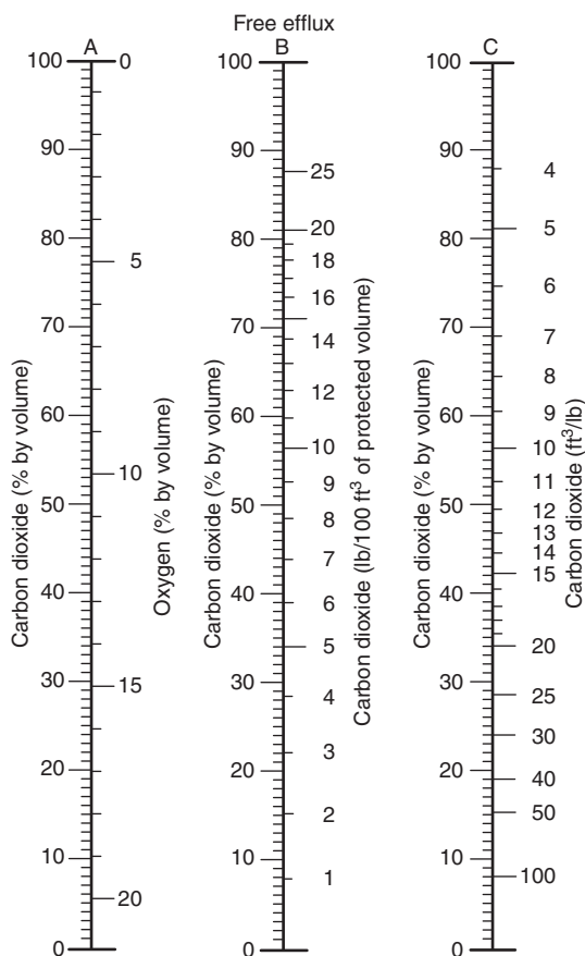
FIGURE D.1(b) Carbon Dioxide Requirements for Inert Atmospheres [based on a carbon dioxide expansion of 8.35 ft³/lb (0.52 m³/kg)].
