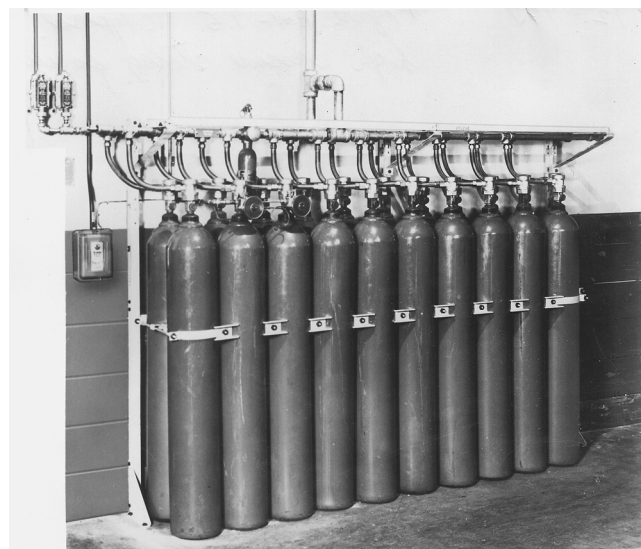
FIGURE A.4.6.5.1 A Typical High-Pressure Storage Facility.
