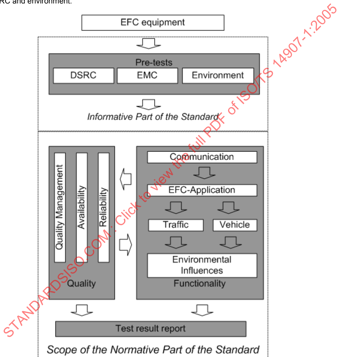
Figure 3 — Test plan - interdependencies
