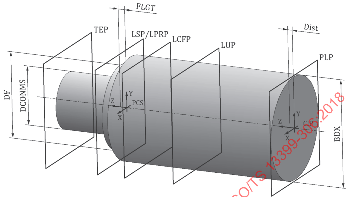
Figure 46 — Outside basic geometry of a trepanning drill
