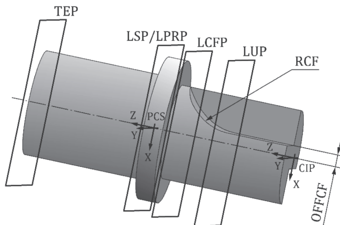
Figure 35 — Chip flute of a face countersinking tool
