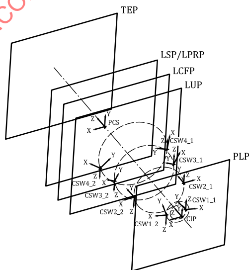
Figure 20 — Determination of coordinate systems of inserts
