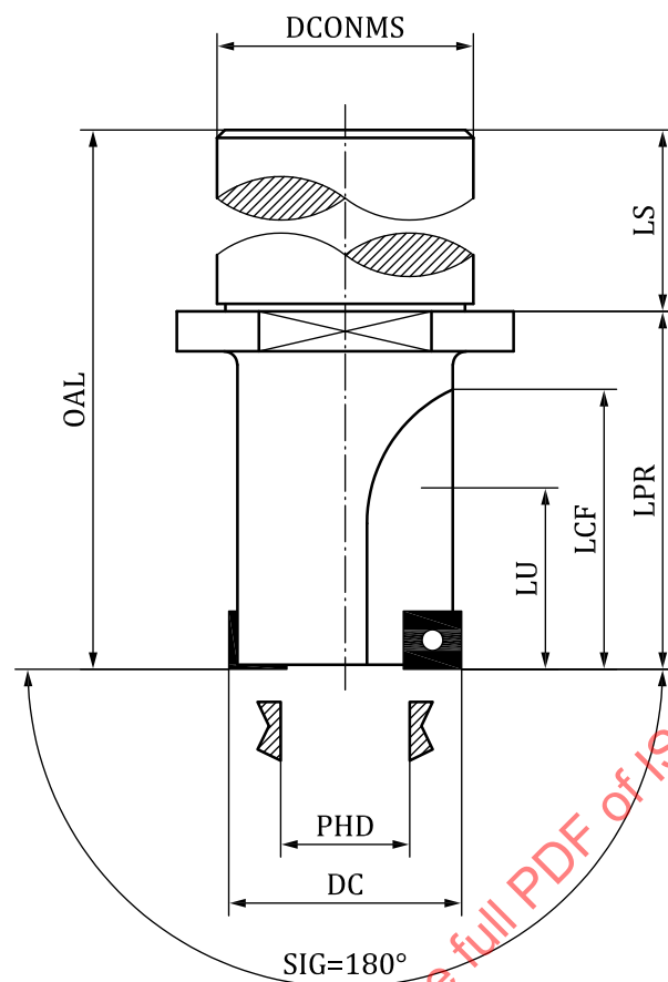
Figure 32 — Determination of properties of a face countersinking tool
