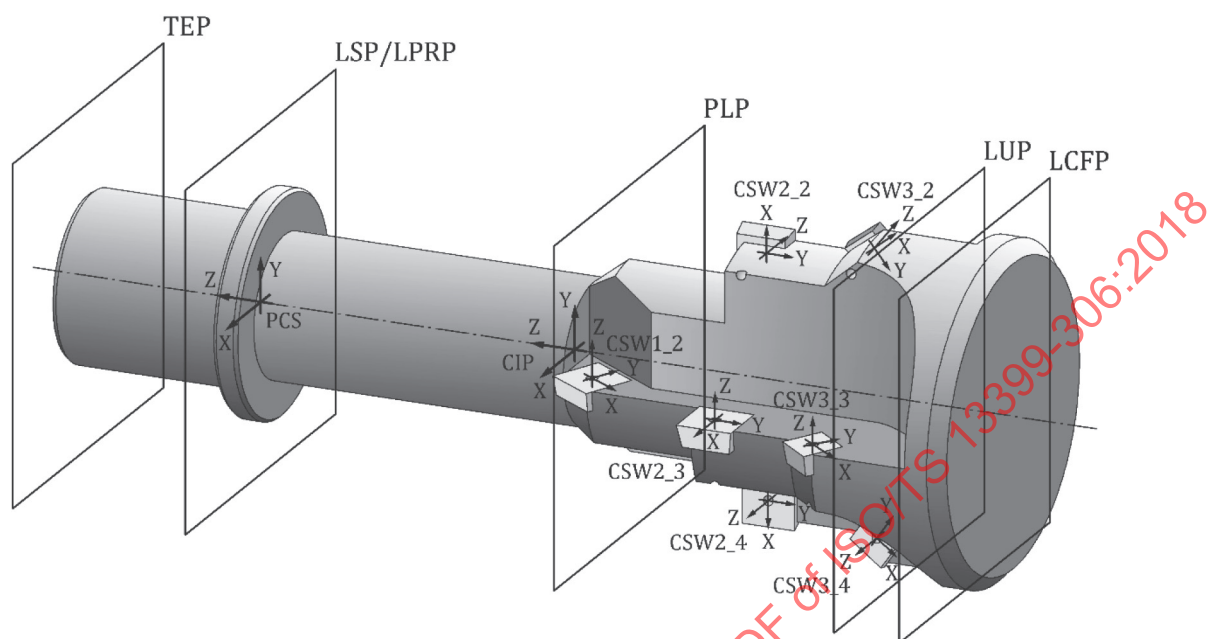
Figure 66 — Determination of CSW's of a reverse countersinking tool
