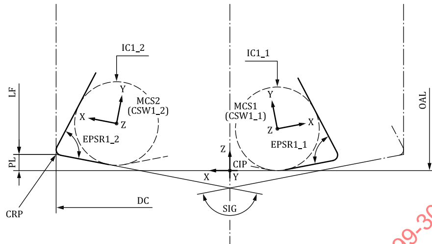
Figure 7 — Determination of CSW x_y for a twist drill
