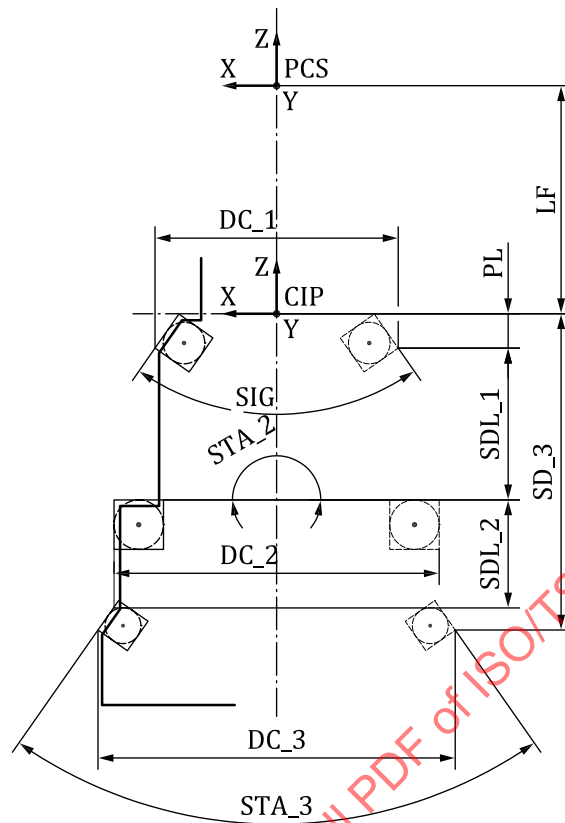
Figure 64 — Determination outside body contour on reverse countersinking tools
