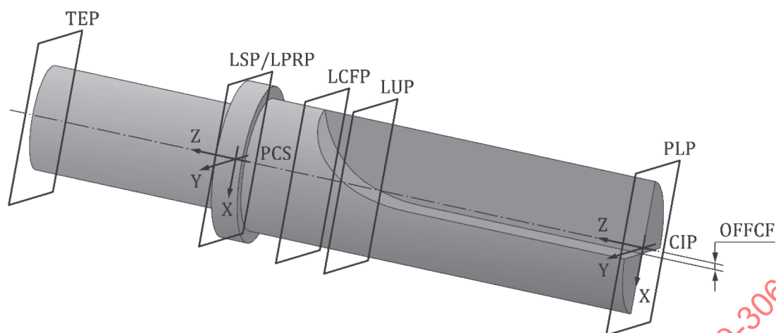
Figure 9 — Chip flute of a twist drill
