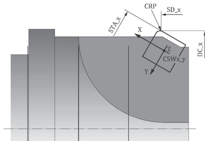
Figure 22 — Pocket seat position of a step drill
