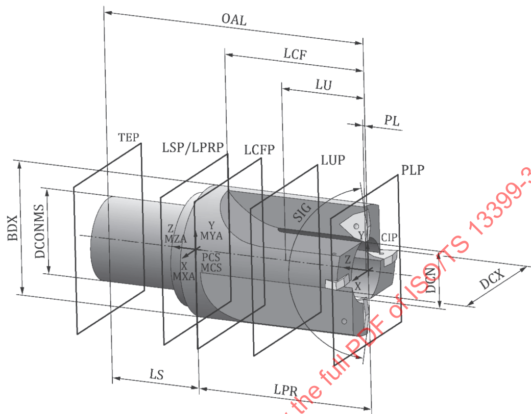
Figure 53 — Assembled trepanning drill
