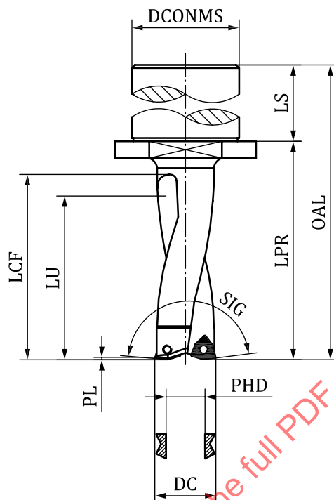
Figure 26 — Determination of properties of a core drill for indexable inserts
