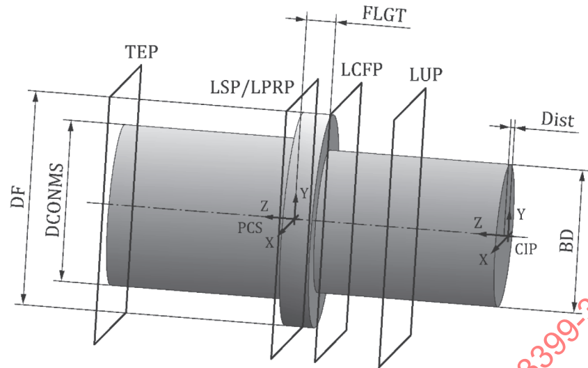
Figure 33 — Basic geometry of a face countersinking tool
