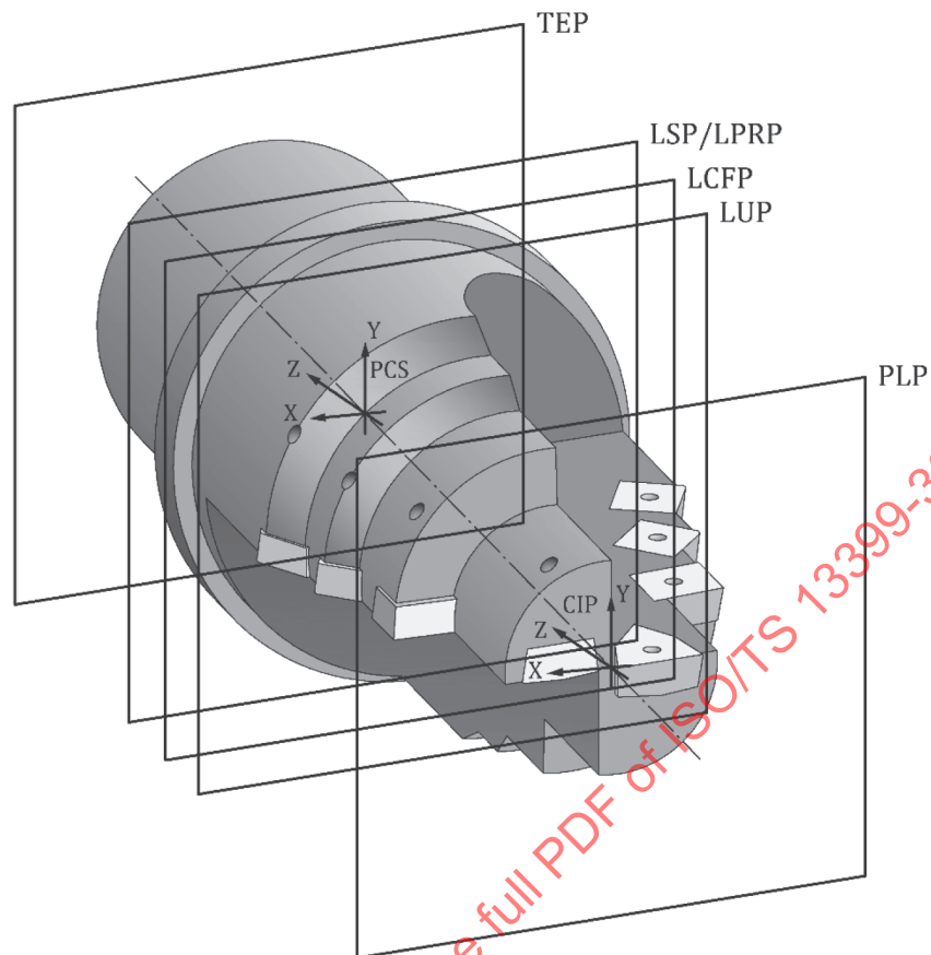
Figure 24 — Position of CRP's on a step drill
