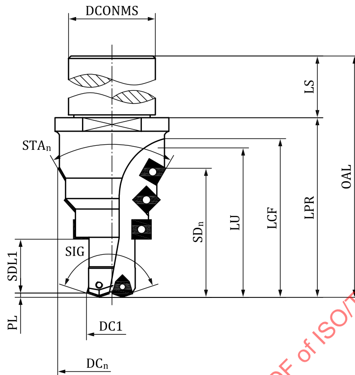
Figure 17 — Determination of properties of step drill for indexable inserts
