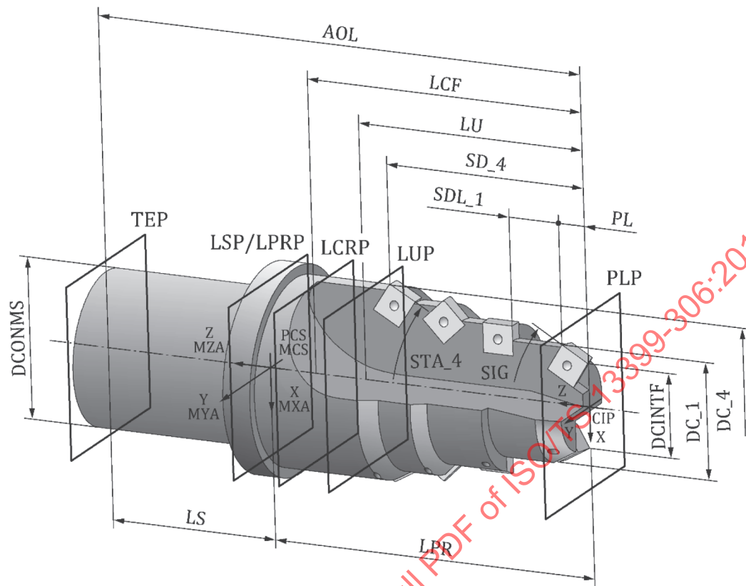
Figure 44 — Assembled step countersinking tool
