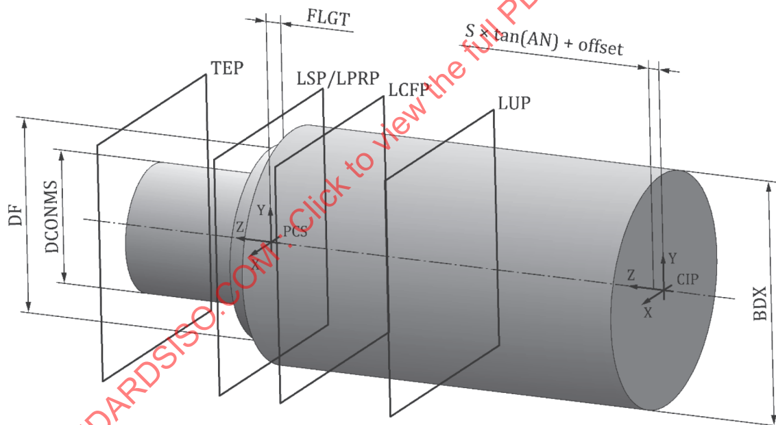
Figure 55 — Outer contour of a bell style countersinking tool
