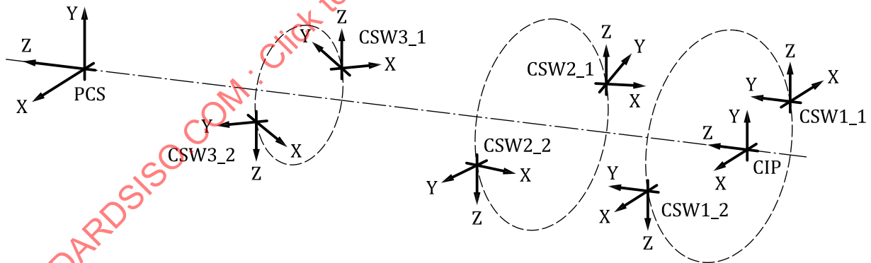
Figure 57 — Determination of CSW's
