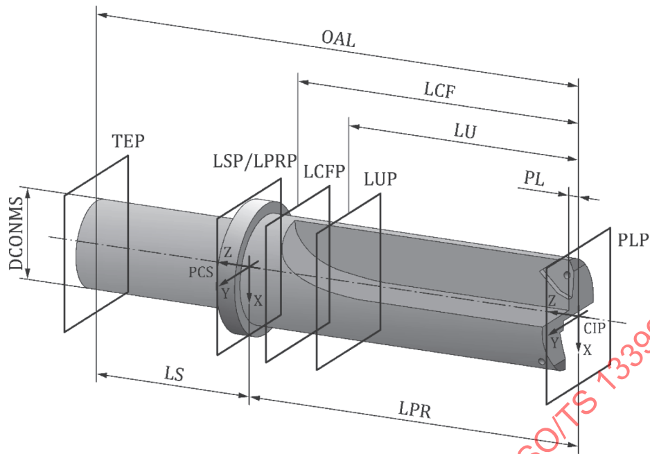
Figure 28 — Basic body of a core drill
