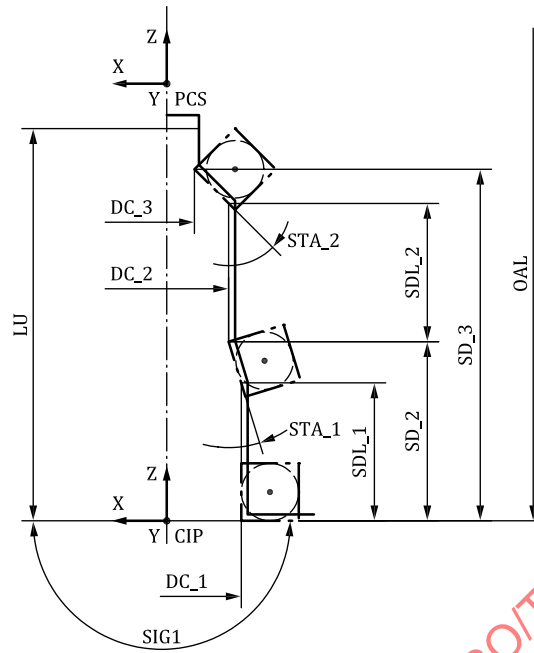
Figure 56 — Determination inside body contour on bell style countersinking tools
