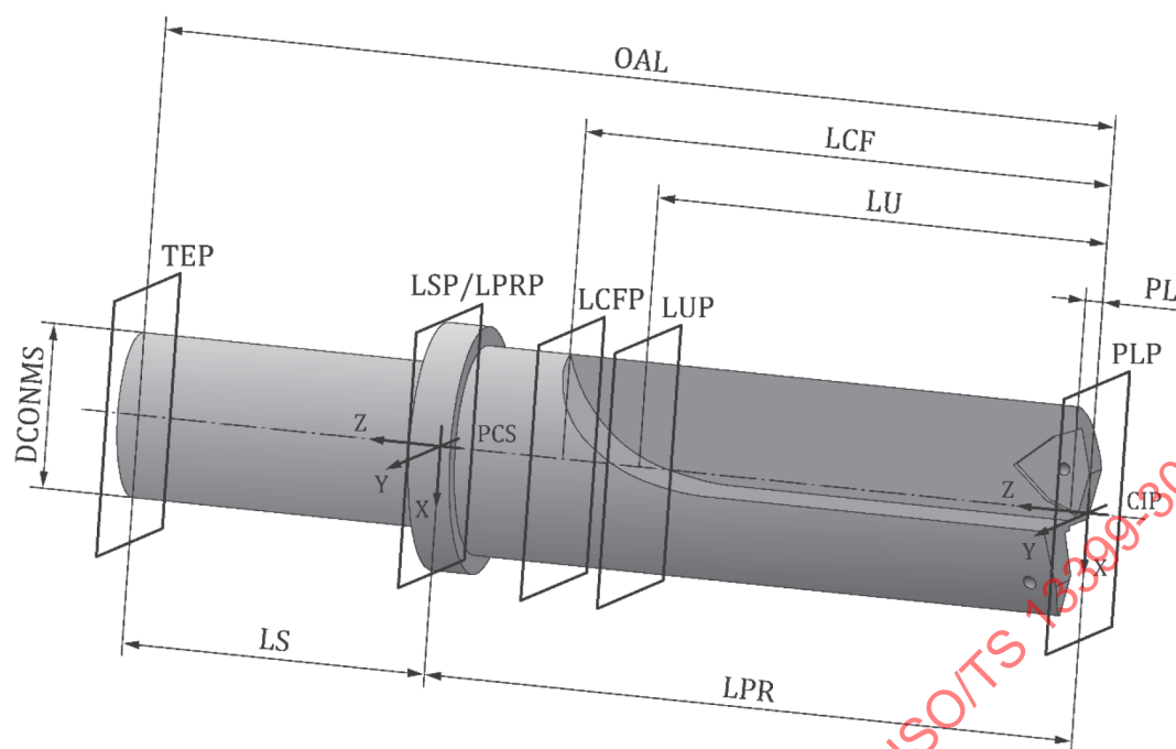
Figure 13 — Twist drill: complete body
