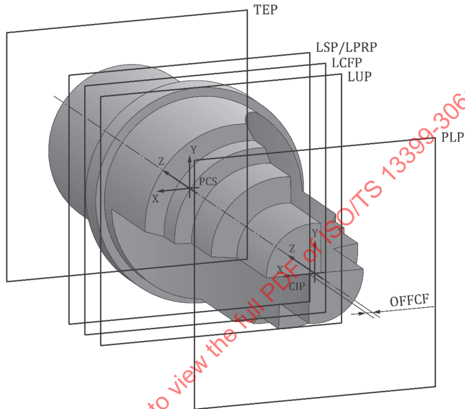
Figure 21 — Step drill: chip flute
