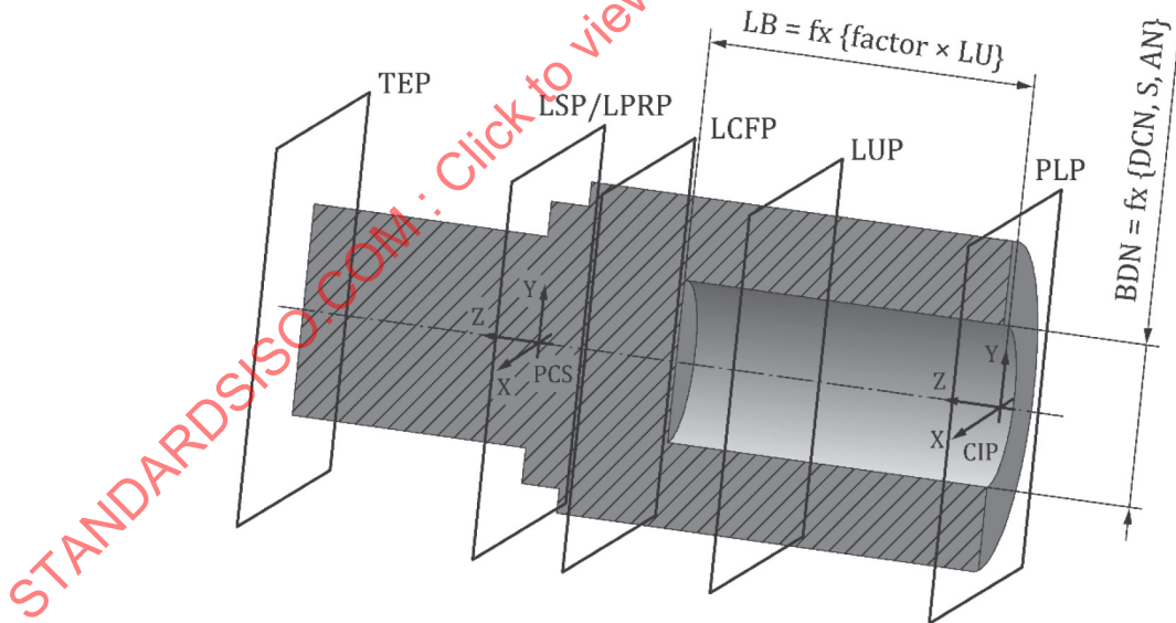
Figure 47 — Inside contour of a trepanning drill
