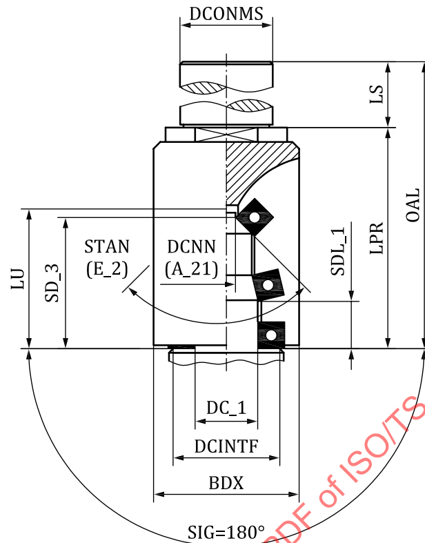
Figure 54 — Determination of properties of a bell style countersinking tool
