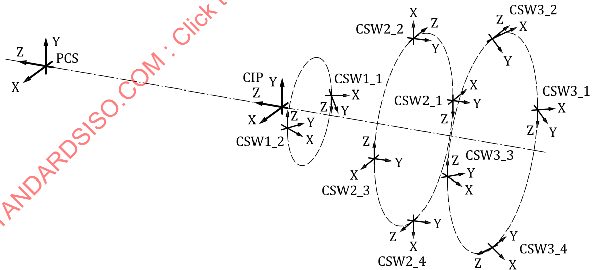
Figure 65 — Determination of CSW's
