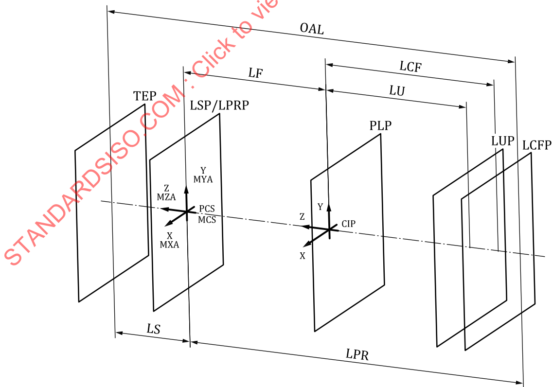
Figure 62 — Determination of planes and properties of a reverse countersinking tool
