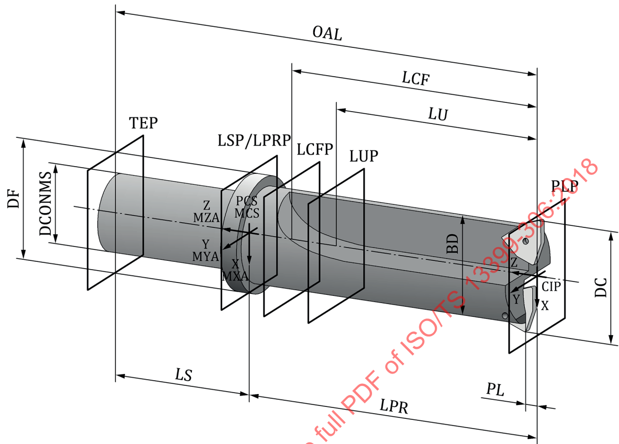
Figure 31 — Assembled core drill
