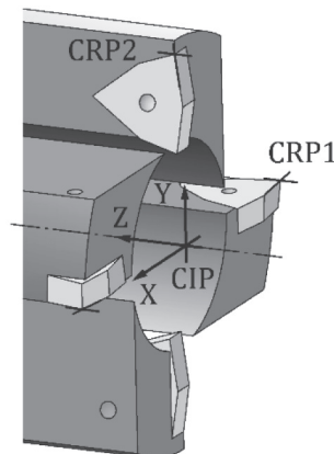
Figure 52 — Trepanning drill: position of CRP's
