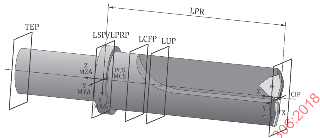
Figure 2 — Example of orientation of "PCS" and "MCS" reference system
