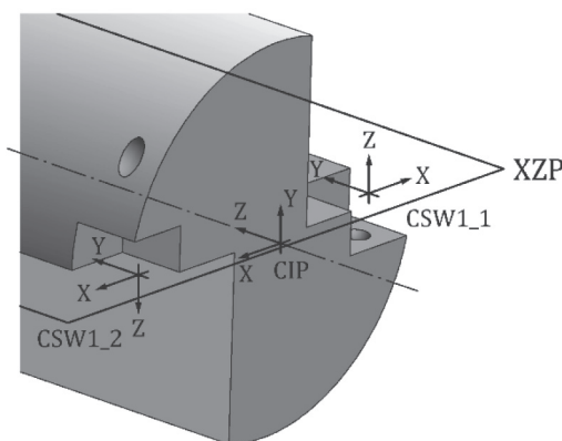
Figure 37 — Position of CSW's
