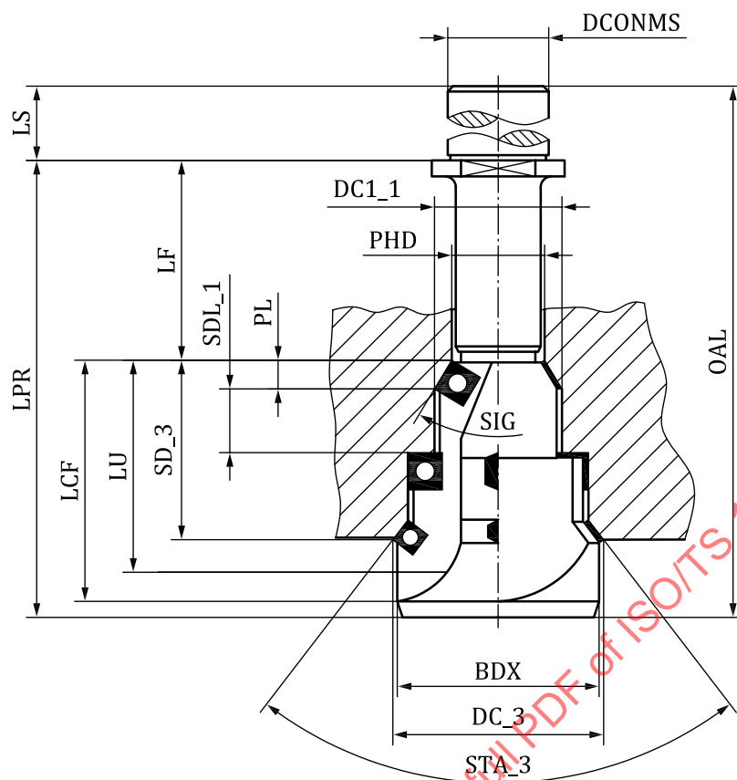
Figure 61 — Determination of properties of a reverse countersinking tool
