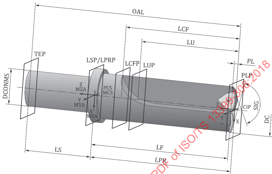
Figure 16 — Example of assembled twist drill
