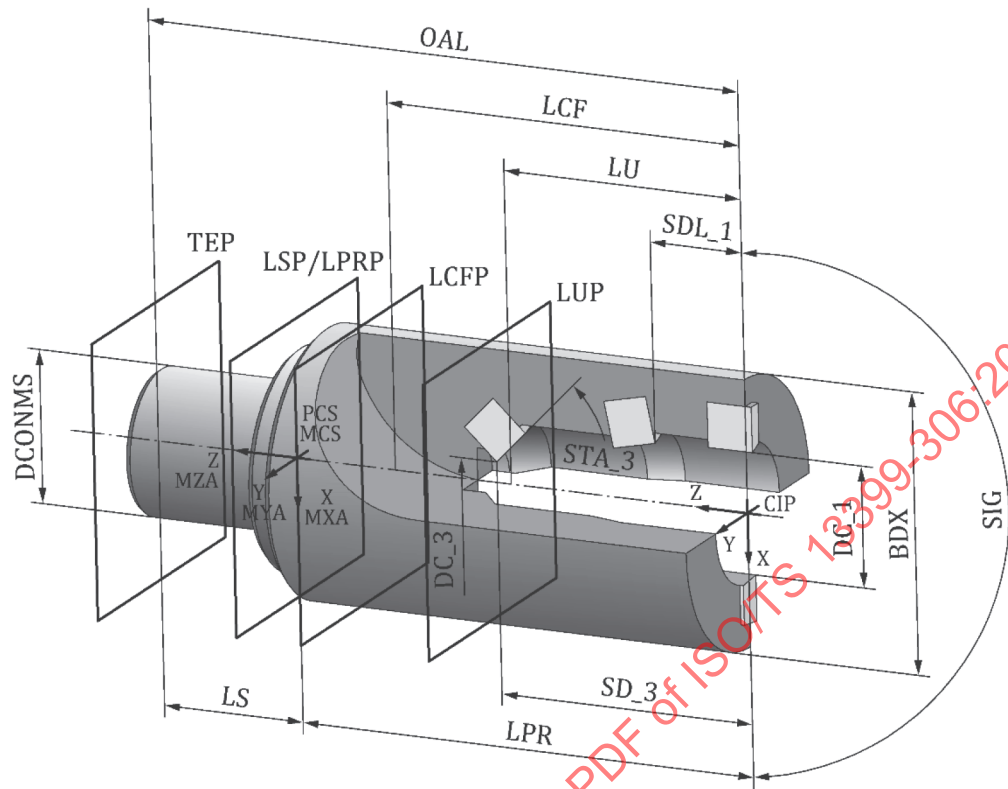
Figure 60 — Assembled bell style countersinking tool
