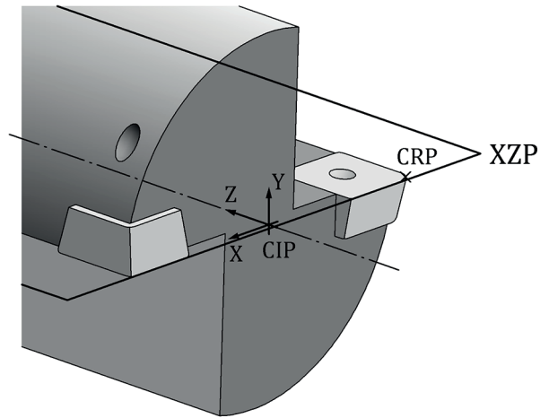
Figure 38 — Position of CRP
