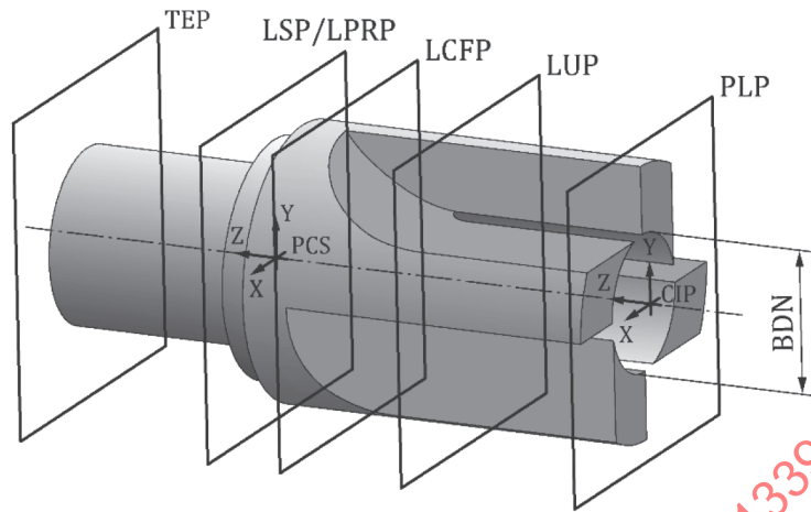
Figure 50 — Arrangement of chip flutes of a trepanning drill
