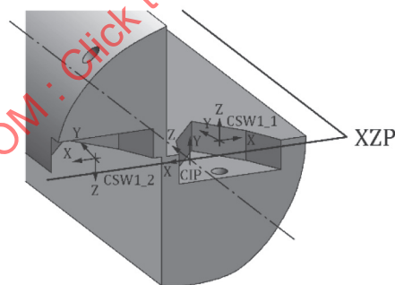
Figure 14 — Position of CSWx_y
