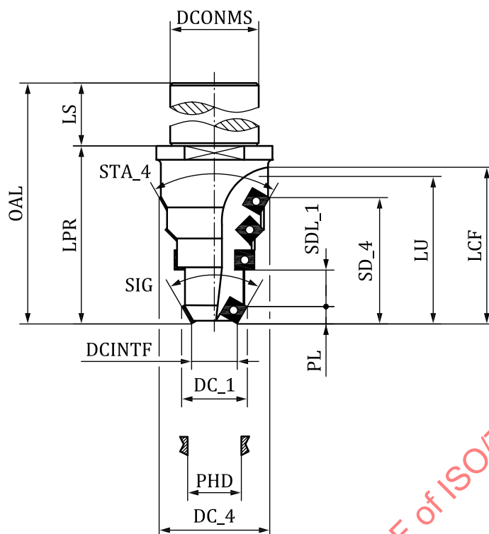
Figure 40 — Determination of properties of step countersinking tool
