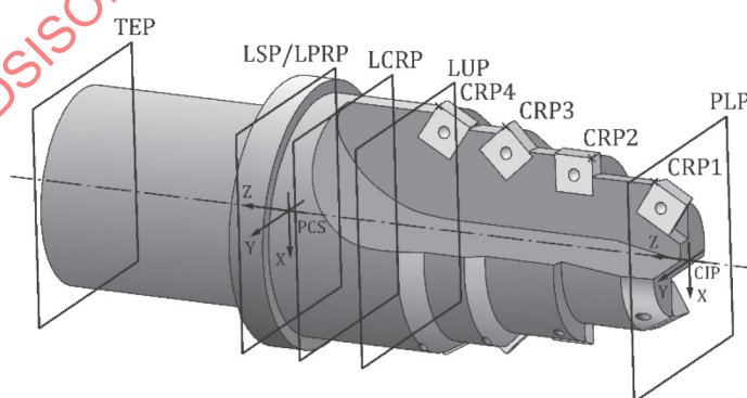
Figure 43 — Position of CRP's of a step countersinking tool
