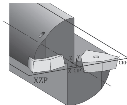
Figure 30 — Position of CRP's of a core drill
