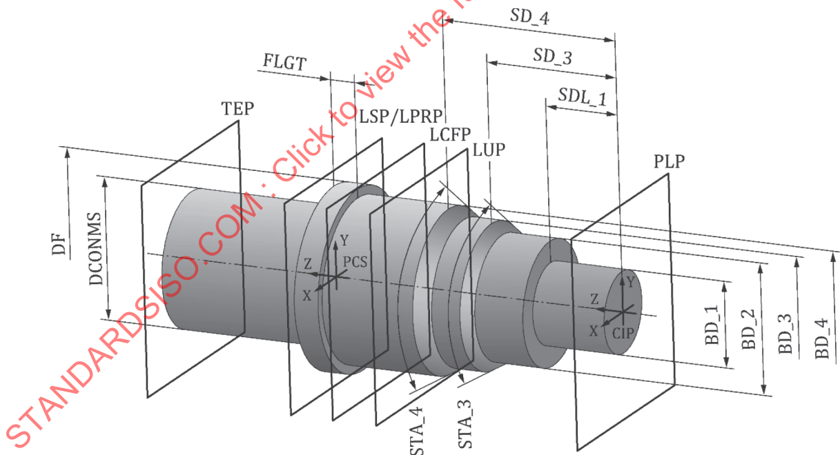
Figure 18 — Basic geometry of a step drill
