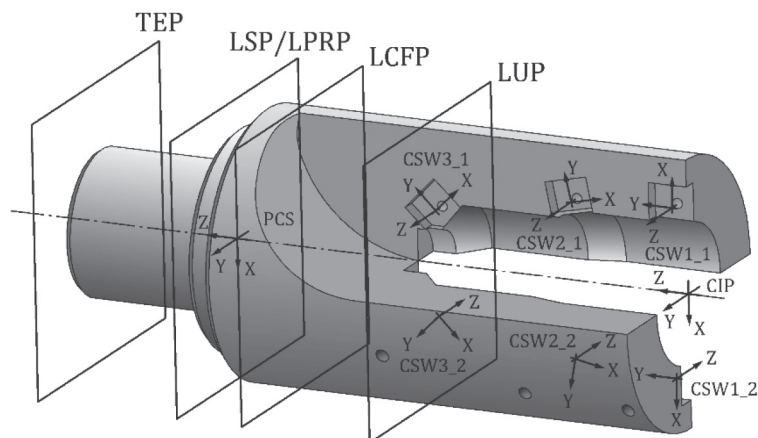
Figure 58 — Position of CSW's of a bell style countersinking tool
