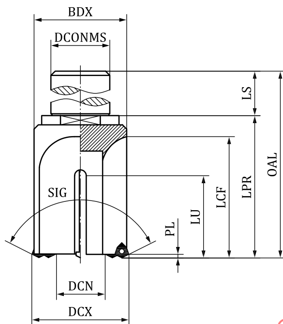
Figure 45 — Determination of properties of a trepanning drill
