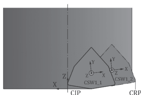
Figure 11 — Inside pocket seat
