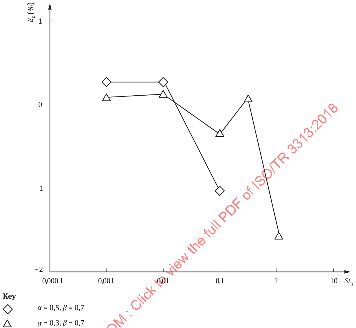
Figure A.2 — Calculated residual error, E_R , for an orifice plate in pulsating flow with corner tappings
