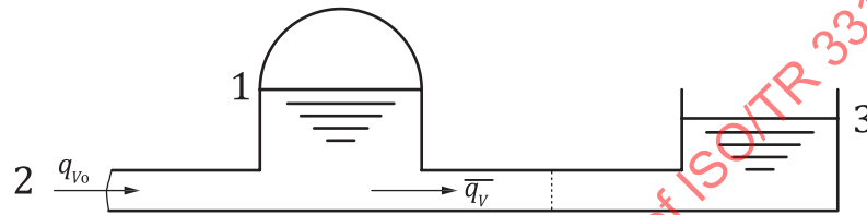
Figure 3 — Use of a surge chamber in pulsating liquid flows
