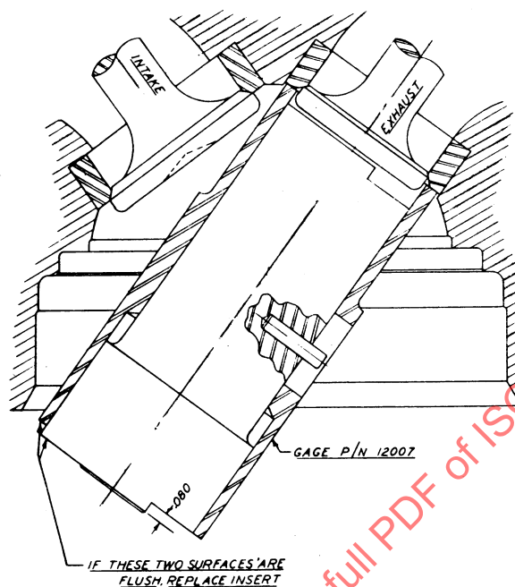
FIGURE 12—METHOD FOR CHECKING EXHAUST VALVE SEATING LIMITS
