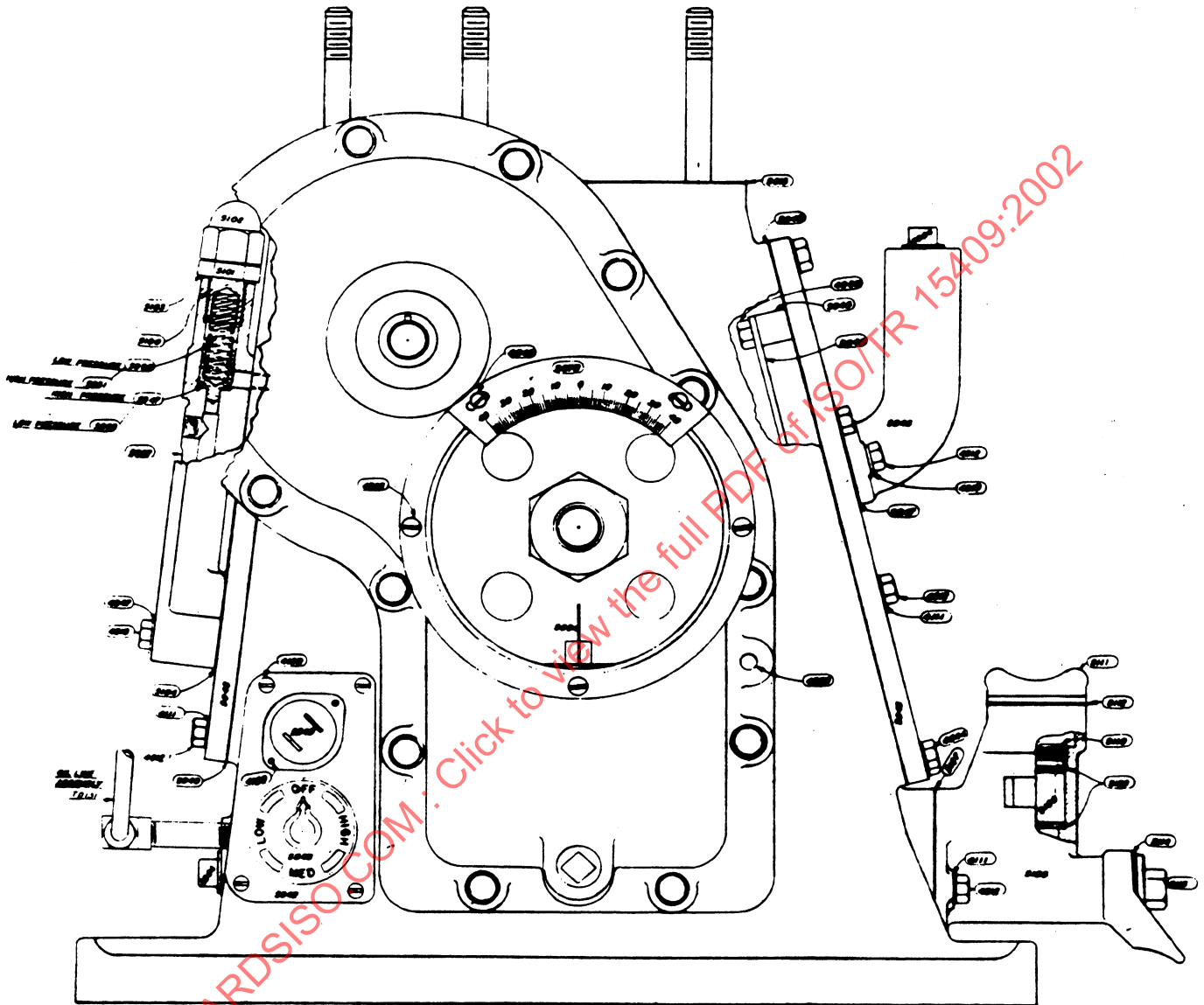
FIGURE 1A—THE 5000 ENGINE
