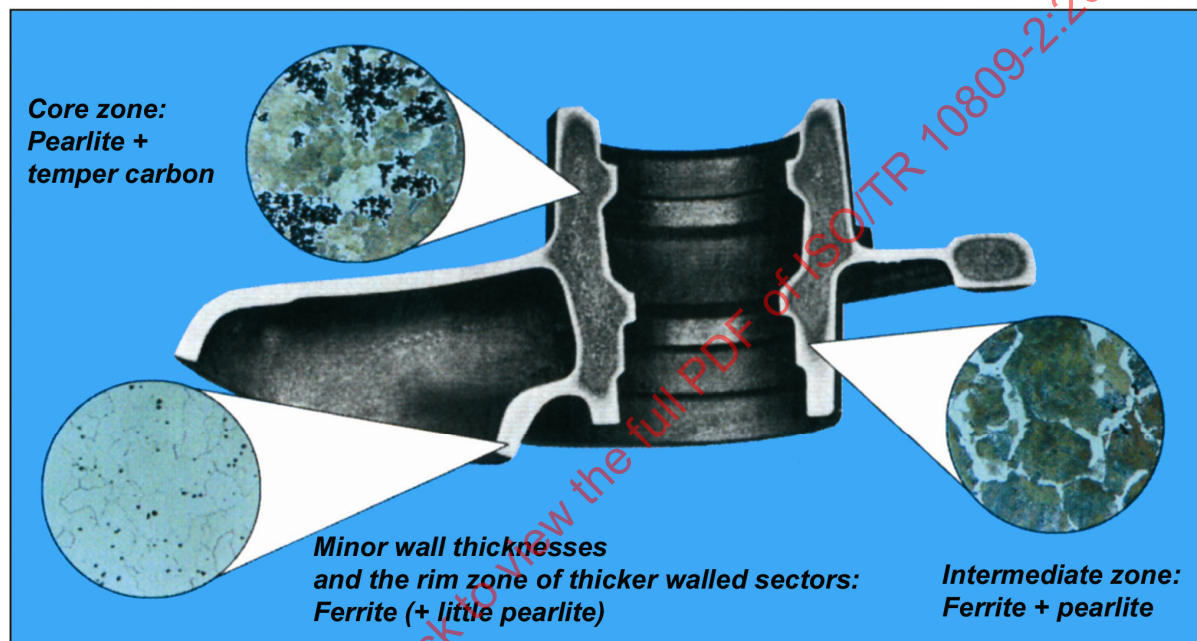
Figure 39 — Microstructure of a whiteheart malleable cast-iron casting
