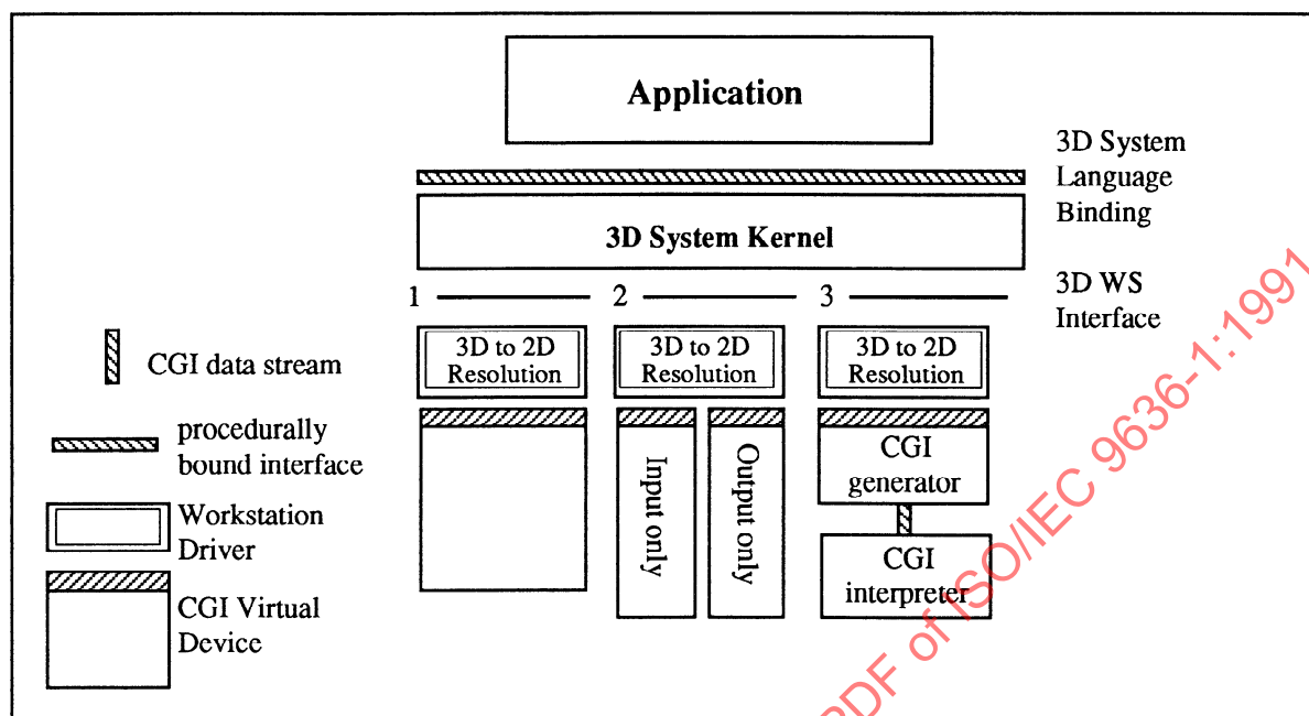
Figure 4 – CGI Virtual Devices as 3D workstations
