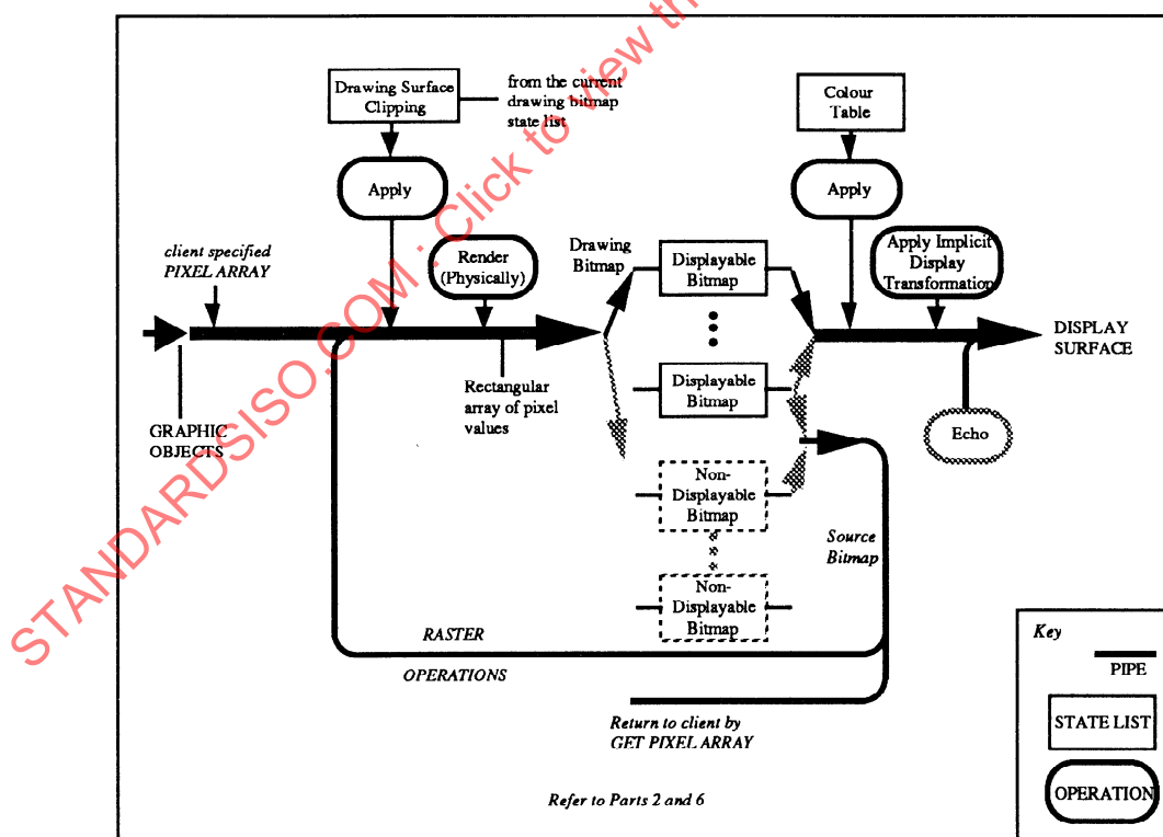
Figure 7 – Additional raster pipeline components
