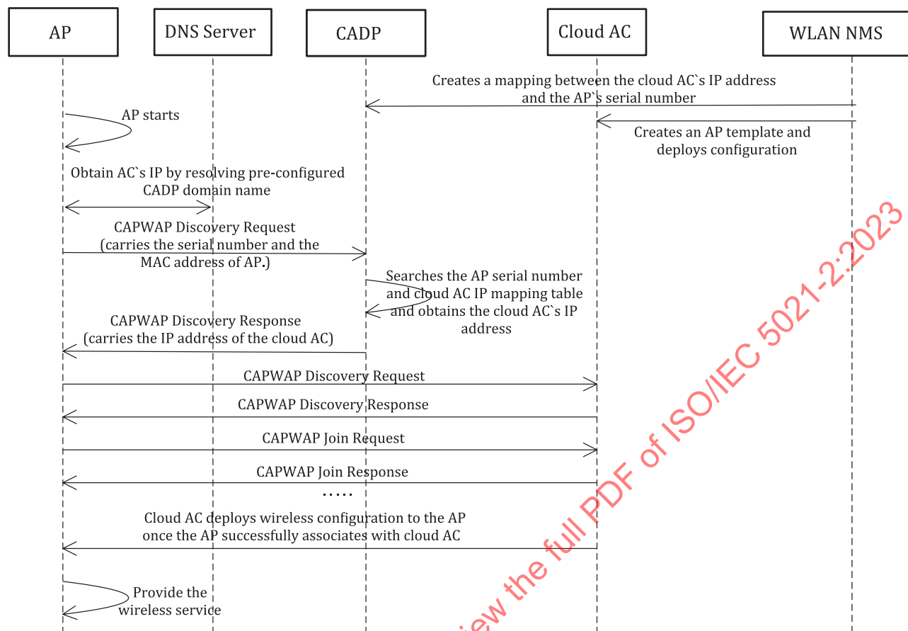
Figure 2 — CACP-based AP association
