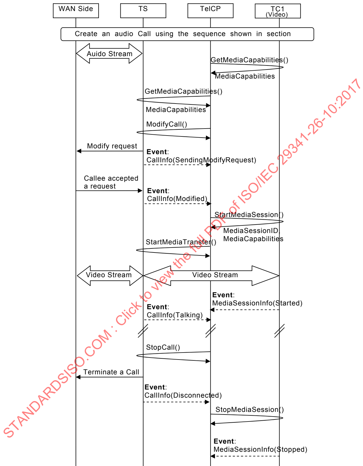
Figure C.6 — Flow basics for modifying an ongoing Call (TS-Based Media Handling)
