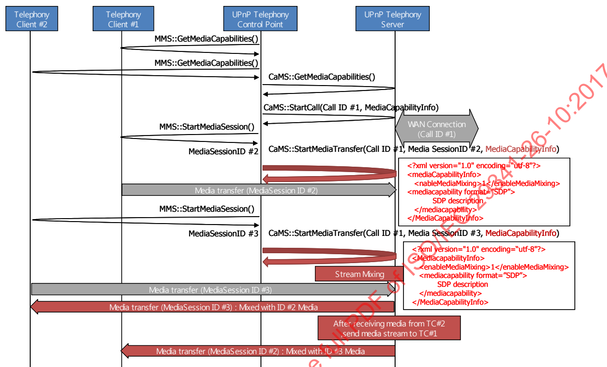
Figure 4 — Starting a Call with Multiple Telephony Clients Using Media Mixing Capability
