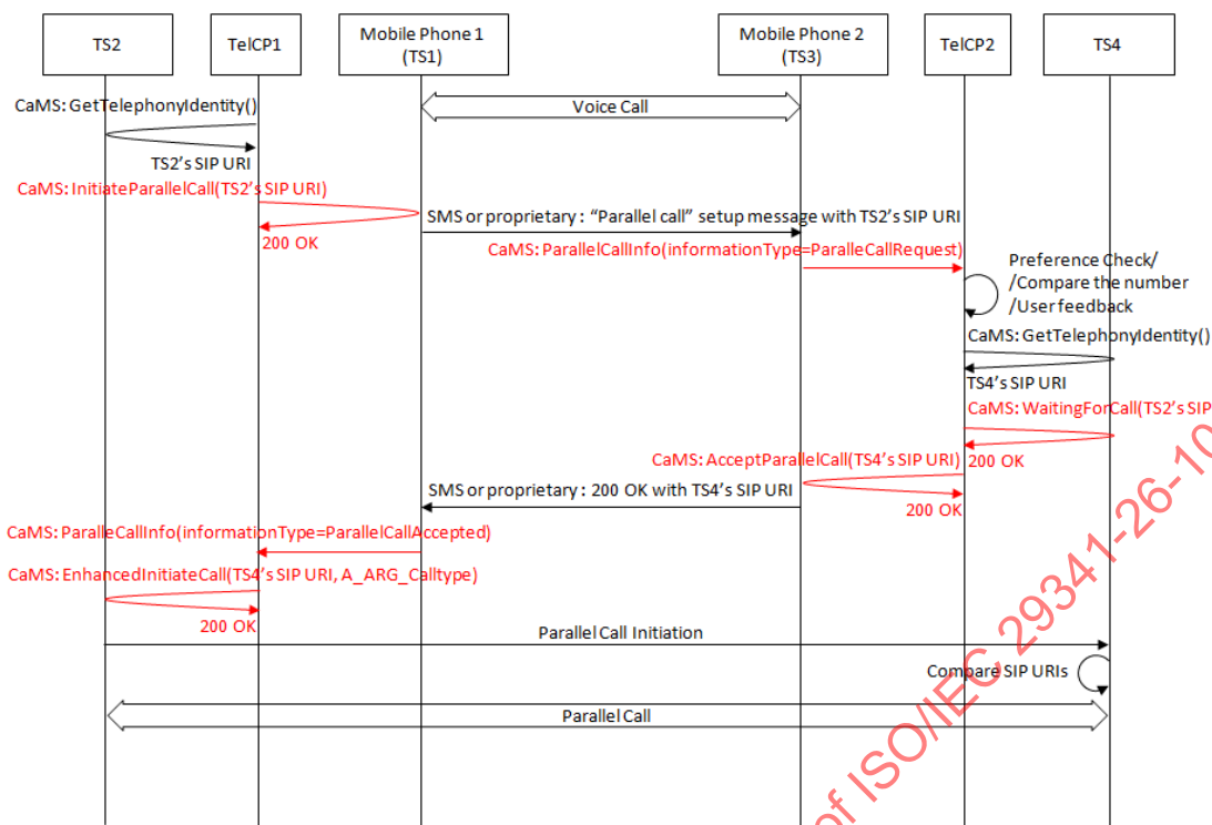
Figure C.16 — Flow basics for Establishing a Parallel Call
