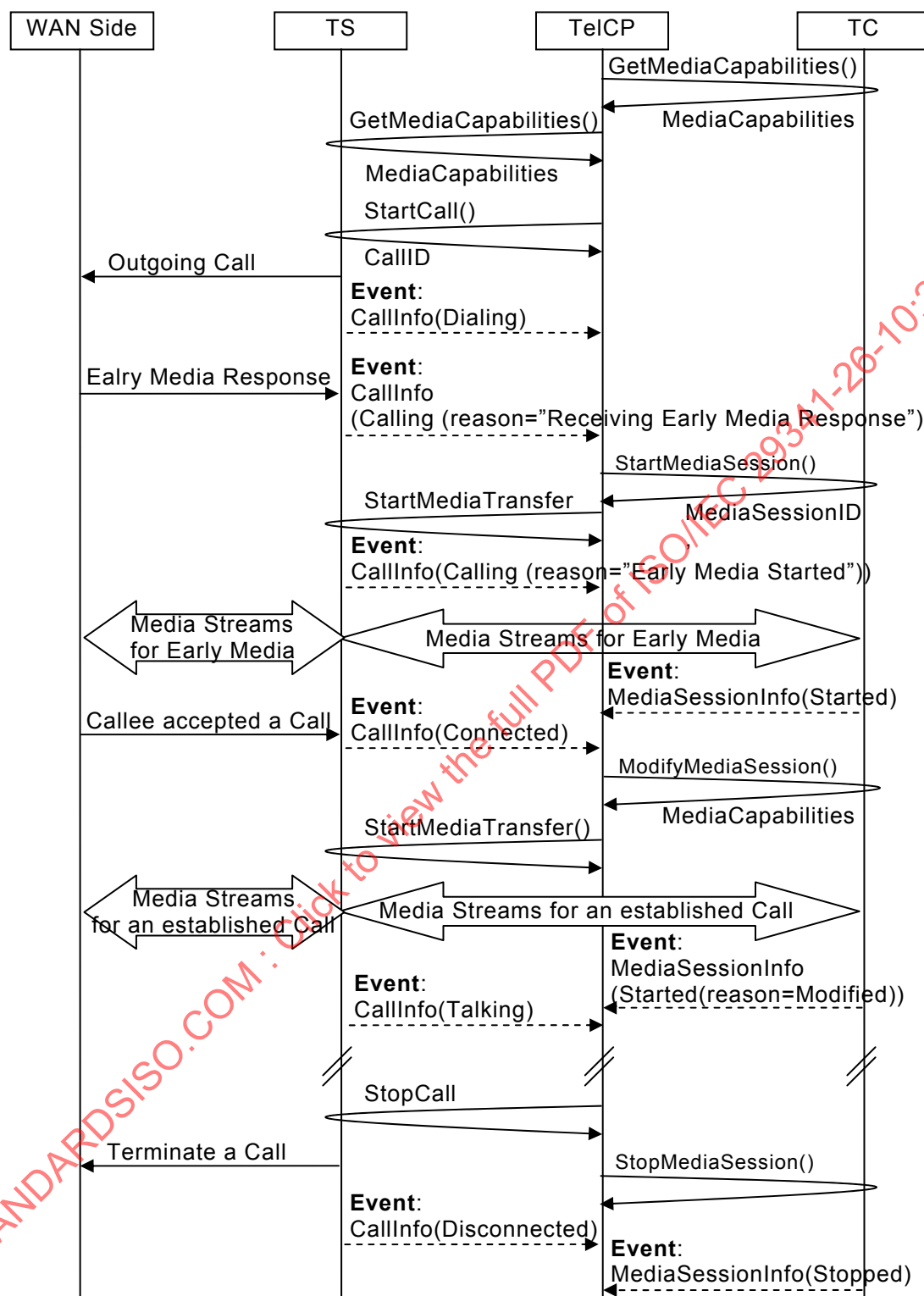
Figure C.9 — Flow basics for Early Media
