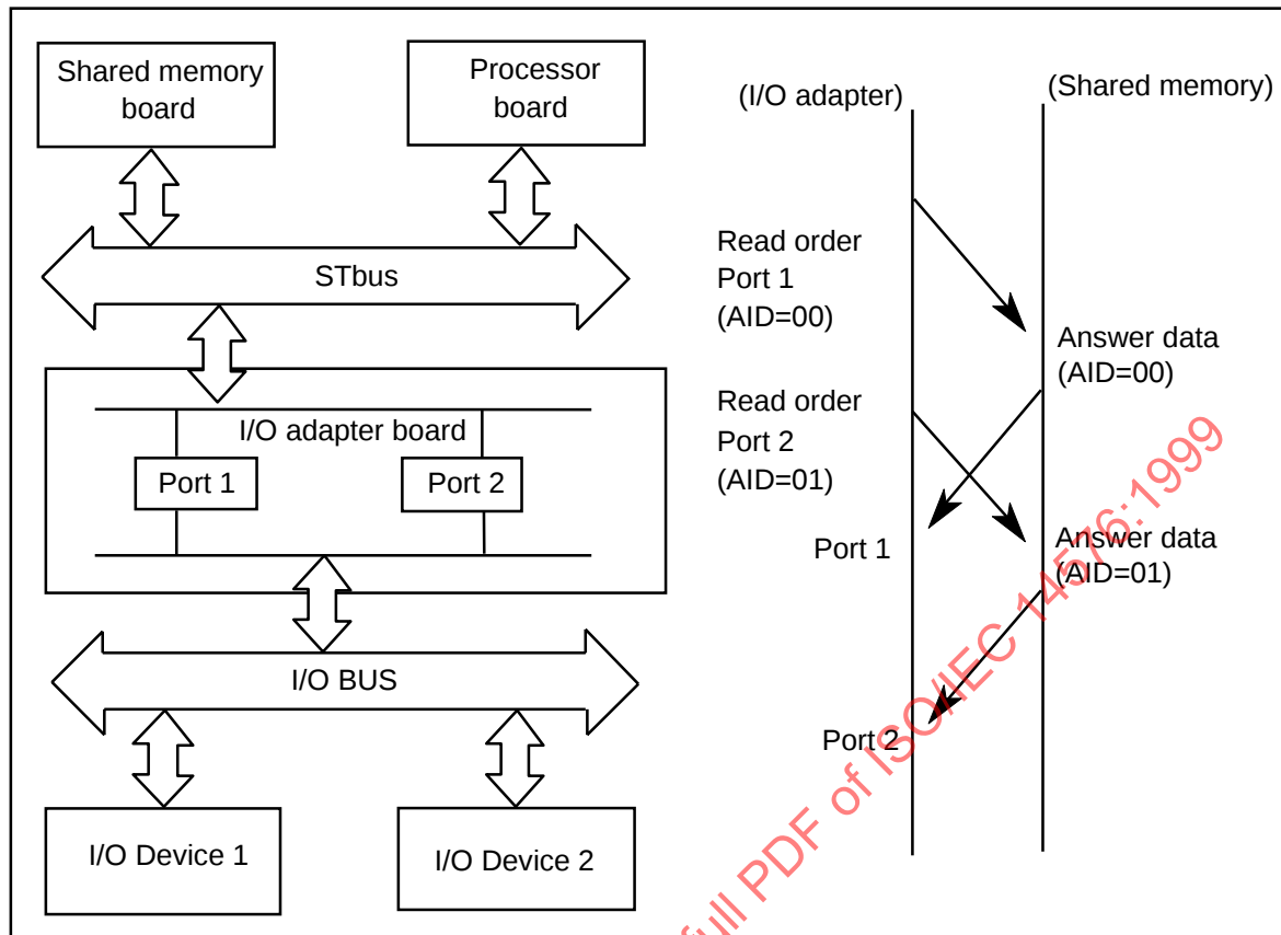
Figure 6 - Pipeline operation
