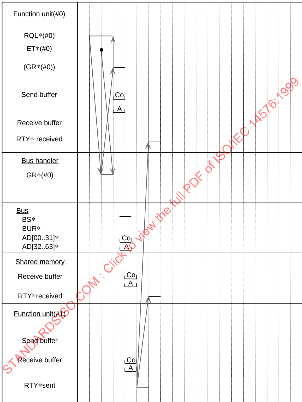
Figure 18 - Retry indication
