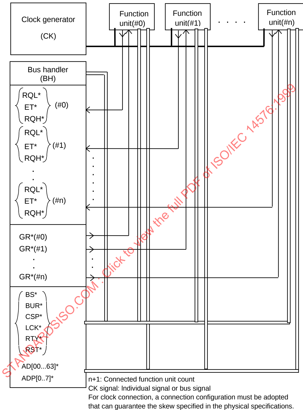
Figure 2 - Connection interface between function units (basic pattern)
