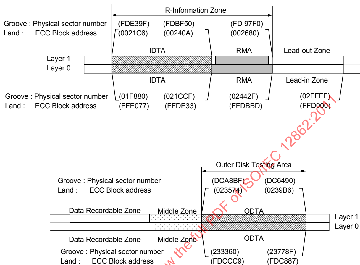
Figure 61 — Address layout of the R-Information Zone and ODTA
