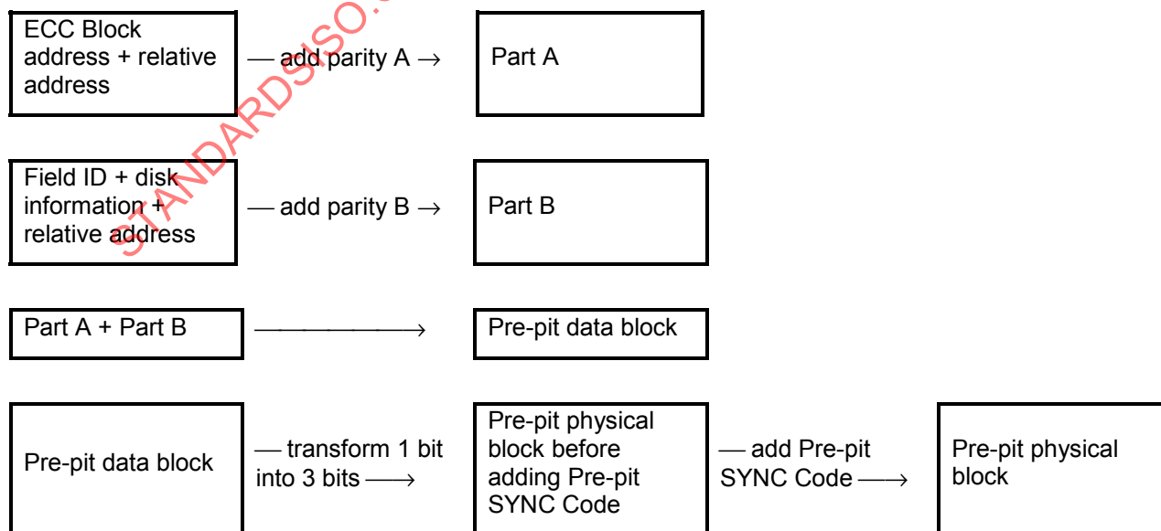
Figure 50 — Processing order to construct a Pre-pit block
