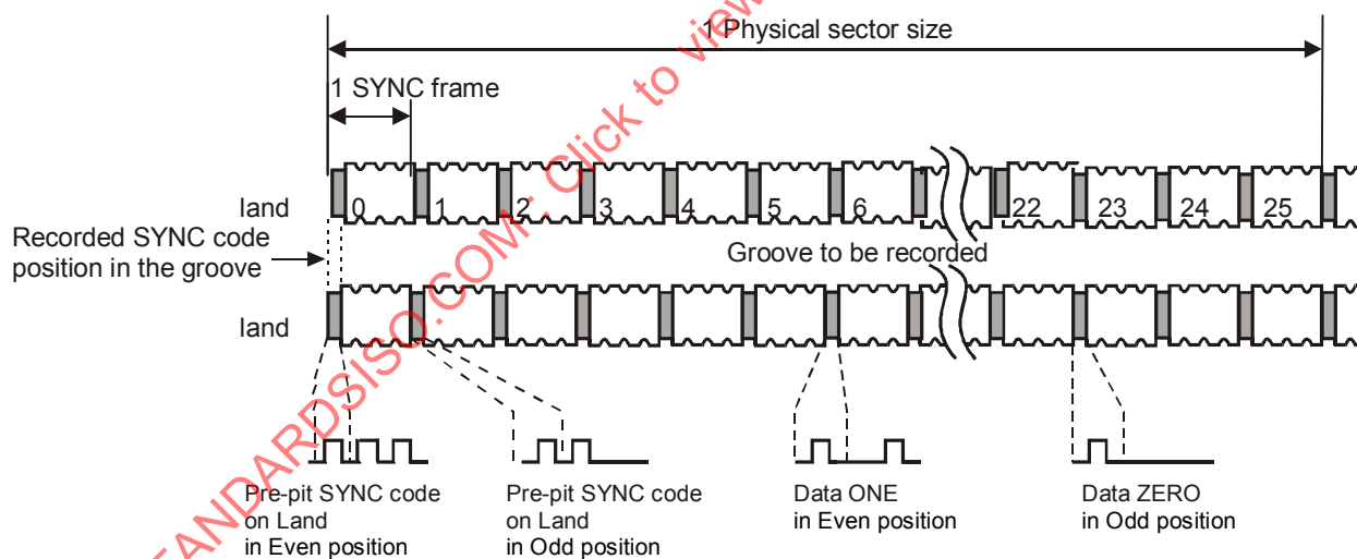
Figure 45 — Track formation
