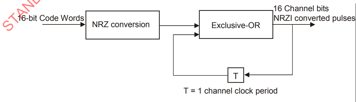
Figure 32 — NRZI conversion
