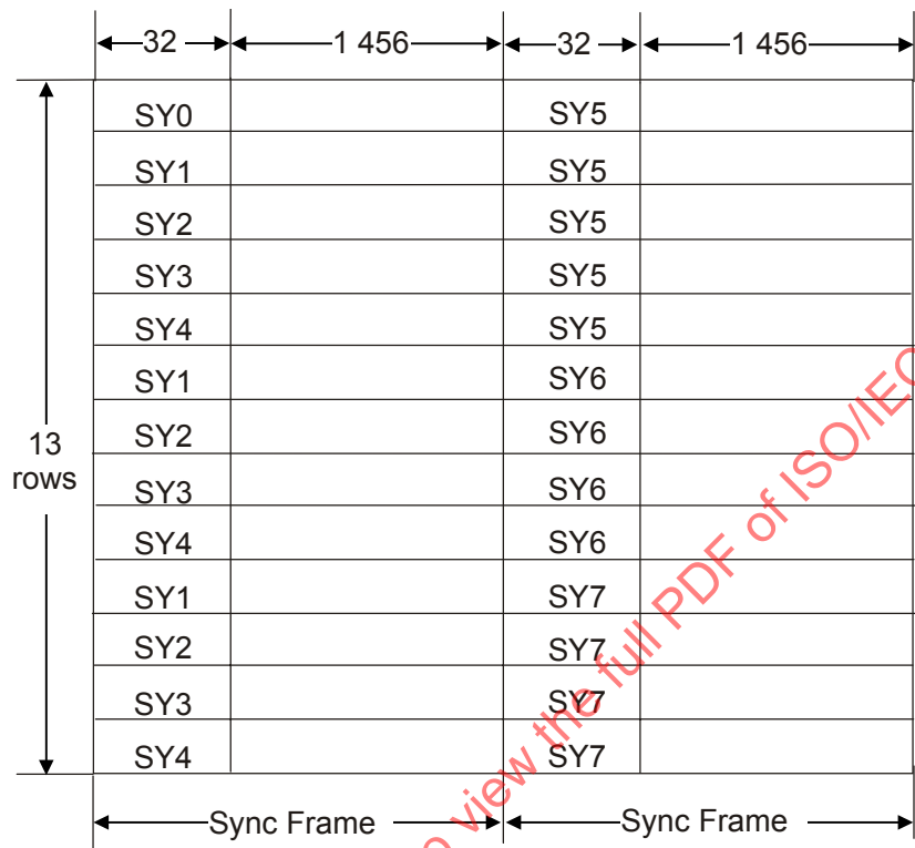
Figure 33 — Physical Sector
