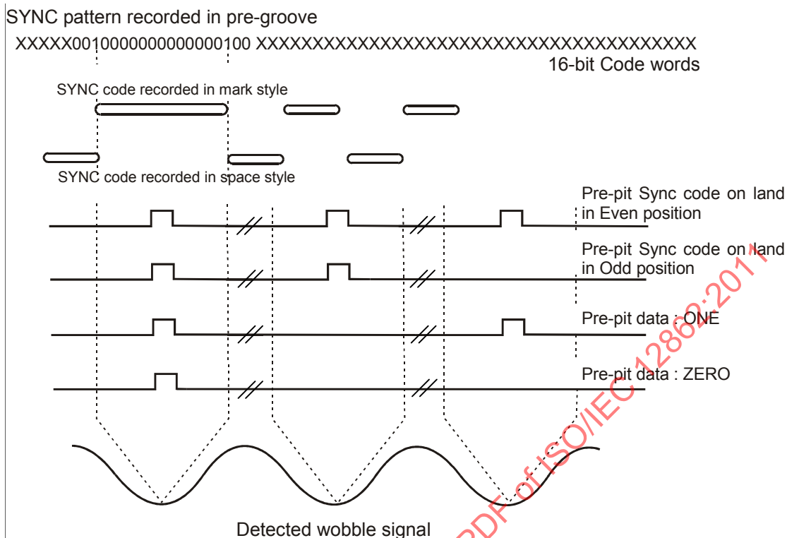
Figure 46 — Relationship of signals recorded in groove and land
