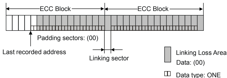
Figure 36 — Structure of ECC Block with Linking Loss Area of 32 768 bytes (32K-Link)
