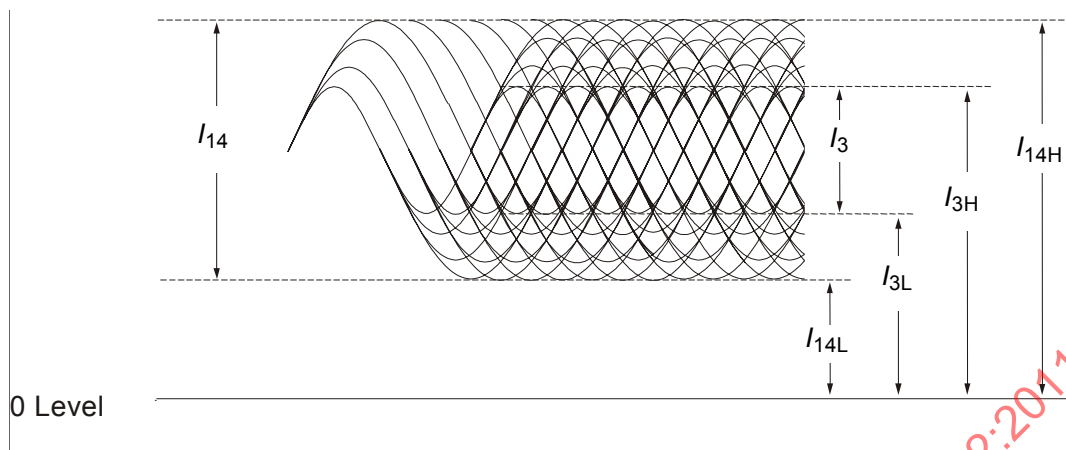
Figure 13 — Modulated amplitude
