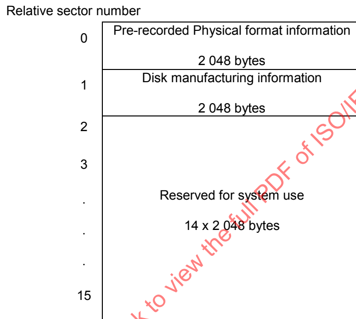
Figure 41 — Structure of a Control data block
