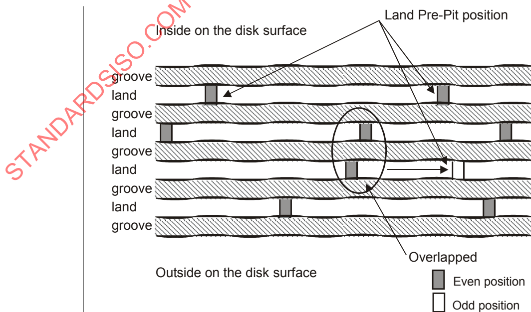
Figure 47 — Layout of land Pre-pit positioning
