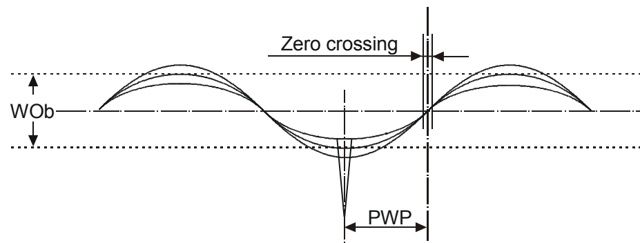
Figure 25 — Relation in phase between wobble and Land Pre-Pit
