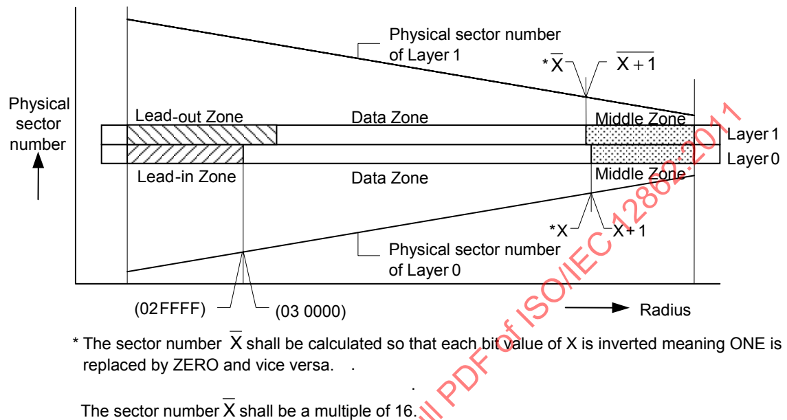
Figure 38 — Physical Sector numbering
