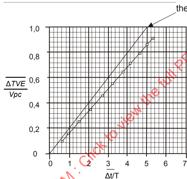
Figure C.2 — Comparator input signal amplitude vs. tracking error signal amplitude
