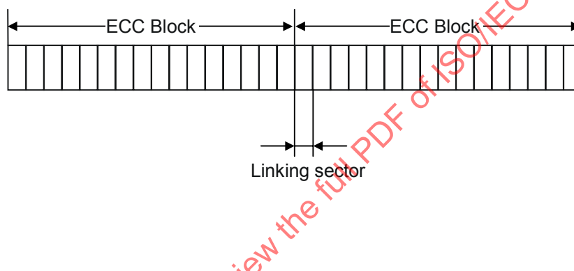
Figure 37 — Structure of ECC Block without Linking Loss Area (Lossless-Link)
