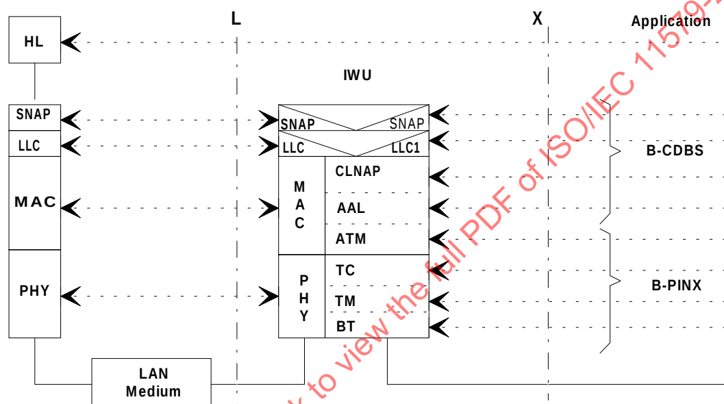
Figure B.1 — Example for conversion functions of an LAN-IWU (bridge-type LAN IWU)
