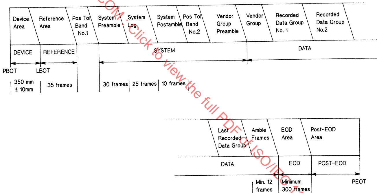
Figure 47- Layout of a Single Data Space tape
