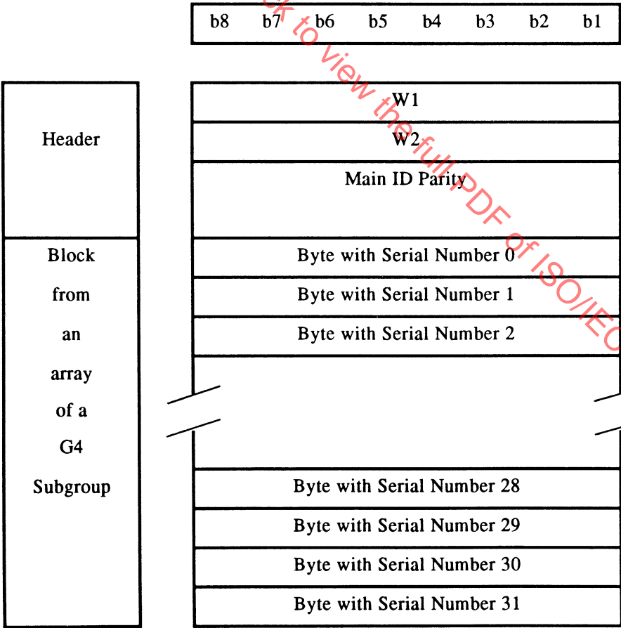
Figure 33 - Main data block
