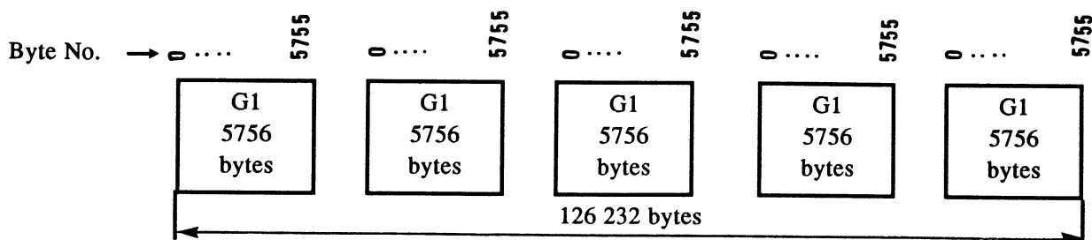
Figure 27 - G1 Sub-Groups
