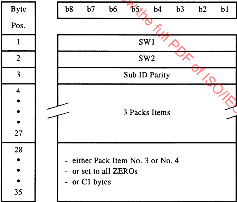
Figure 44 - Sub Data Block
