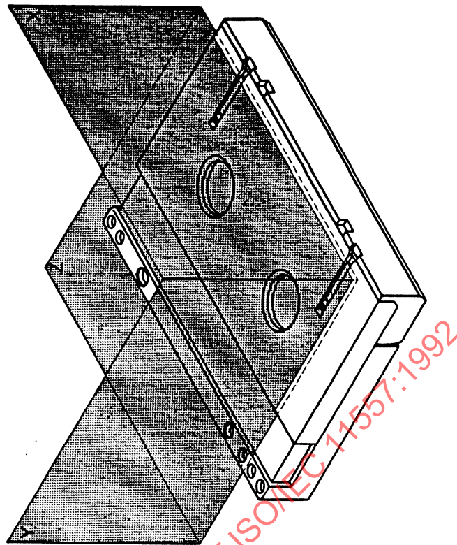
Figure 4 - Reference Planes X, Y, Z
