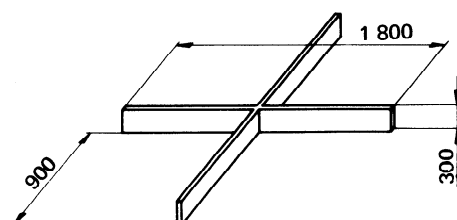
Figure 7 — Quartering irons
