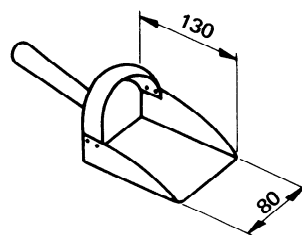
Figure 2 — Hand-scoop
