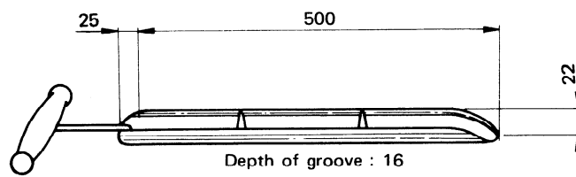
Figure 3 — Divided sampling spear (open trier)
