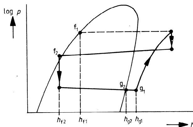
b) Log p versus h diagram
