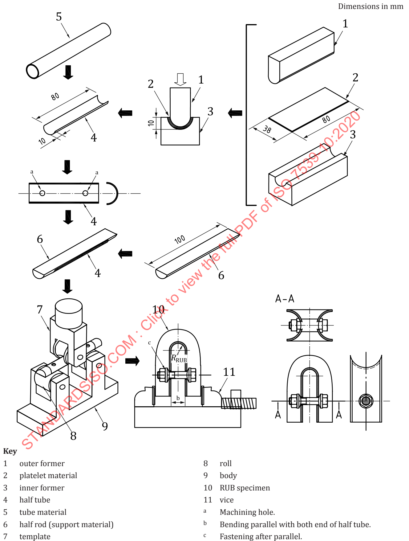
Figure A.2 — Preparation of a non-pre-strained half tube RUB specimen from tubular and plate specimen
