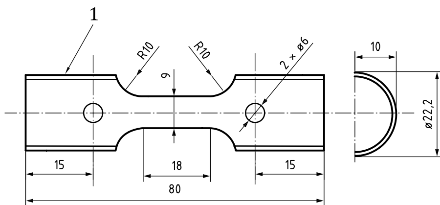
a) Before bending
