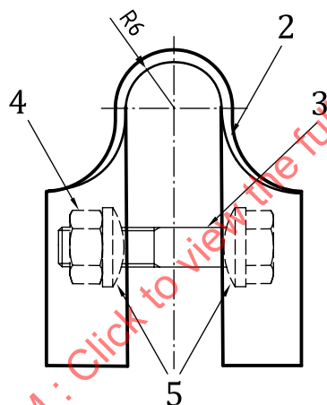
b) After bending
