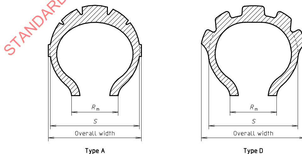
Figure 1 — Tread configurations
