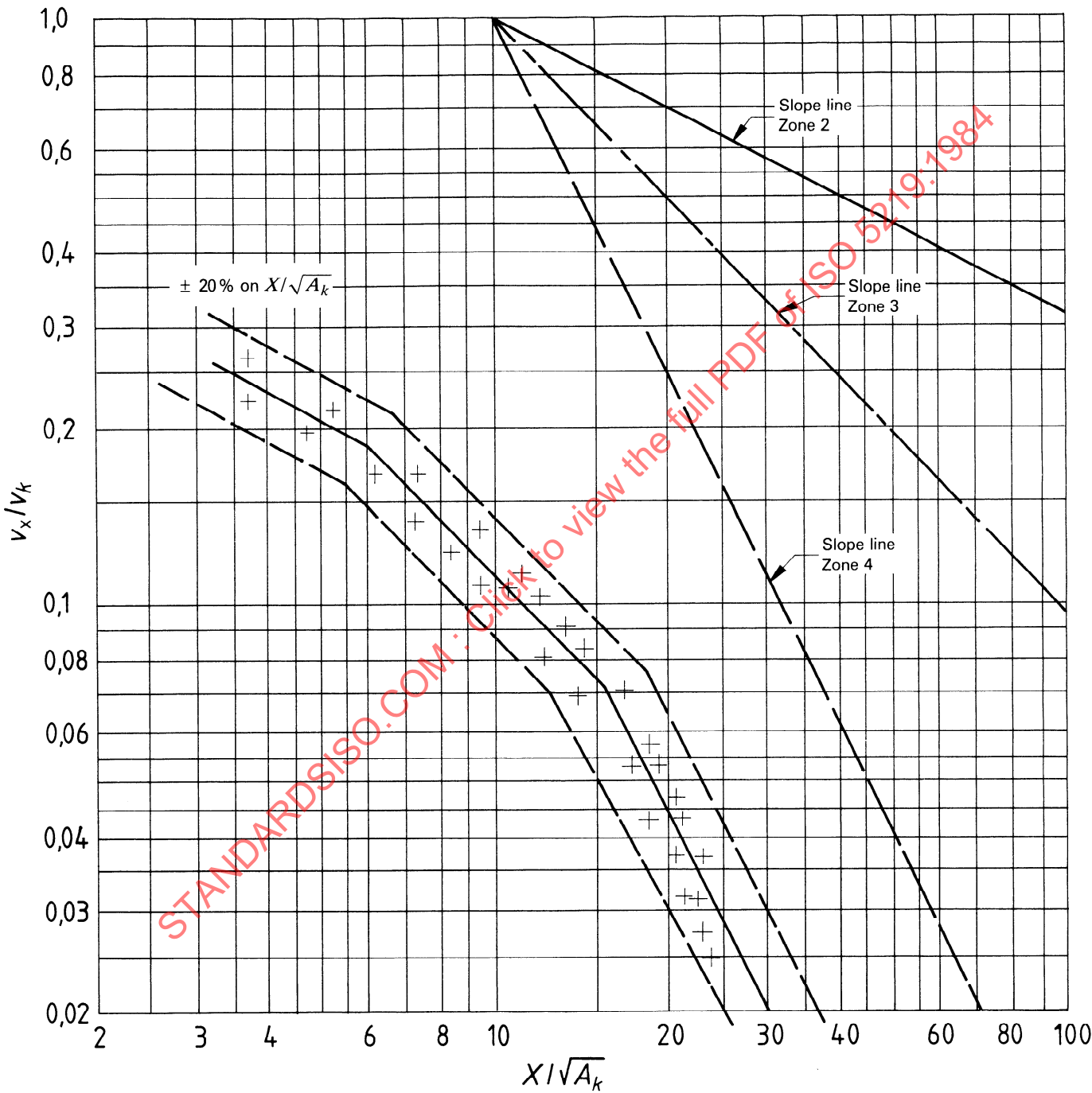
Figure 8 — Typical graph for a family of air terminal devices showing the relationship between throw, reference terminal velocity and air flow rate
