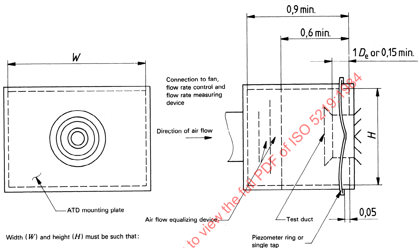
Figure 3 — First test installation: "B" for supply ATD
