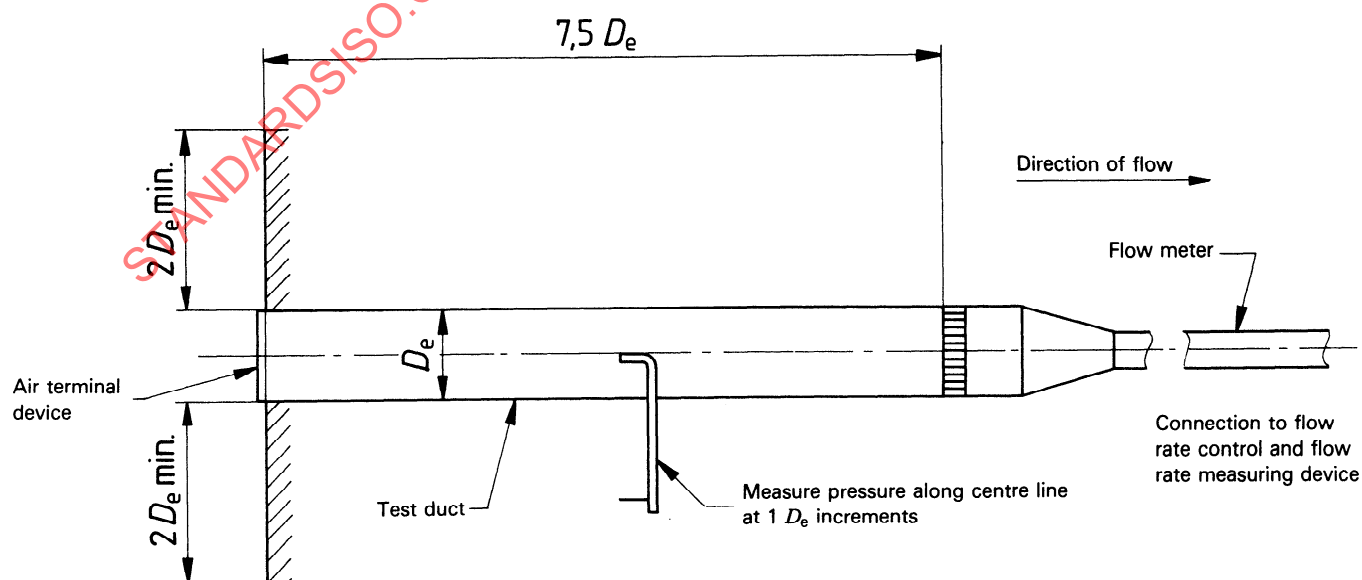
Figure 4 — First test installation "C" for exhaust ATD
