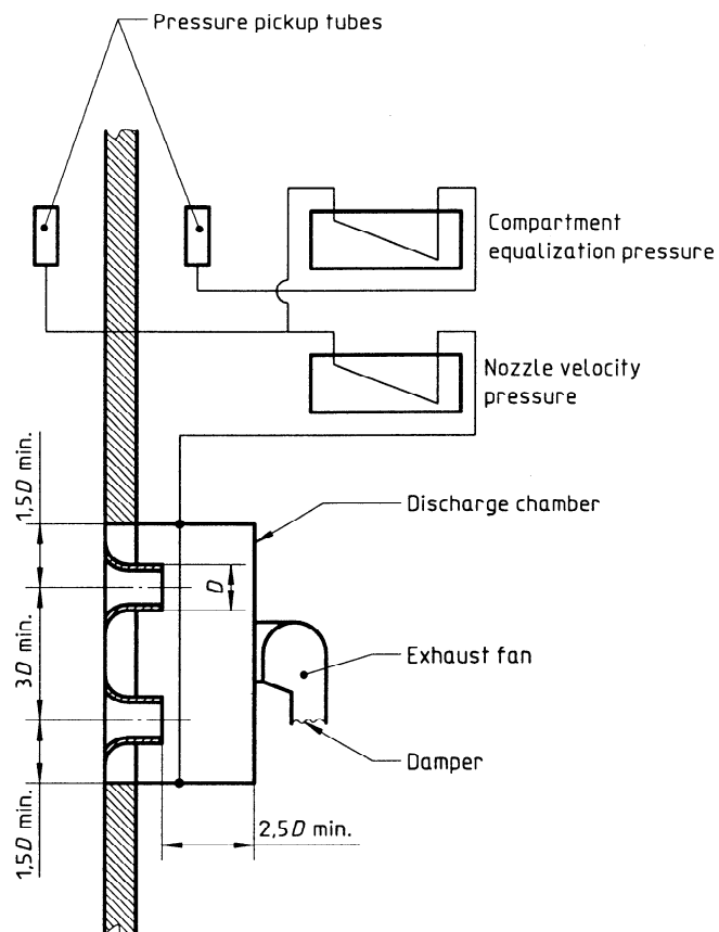
Figure B.1 — Pressure-equalizing device
