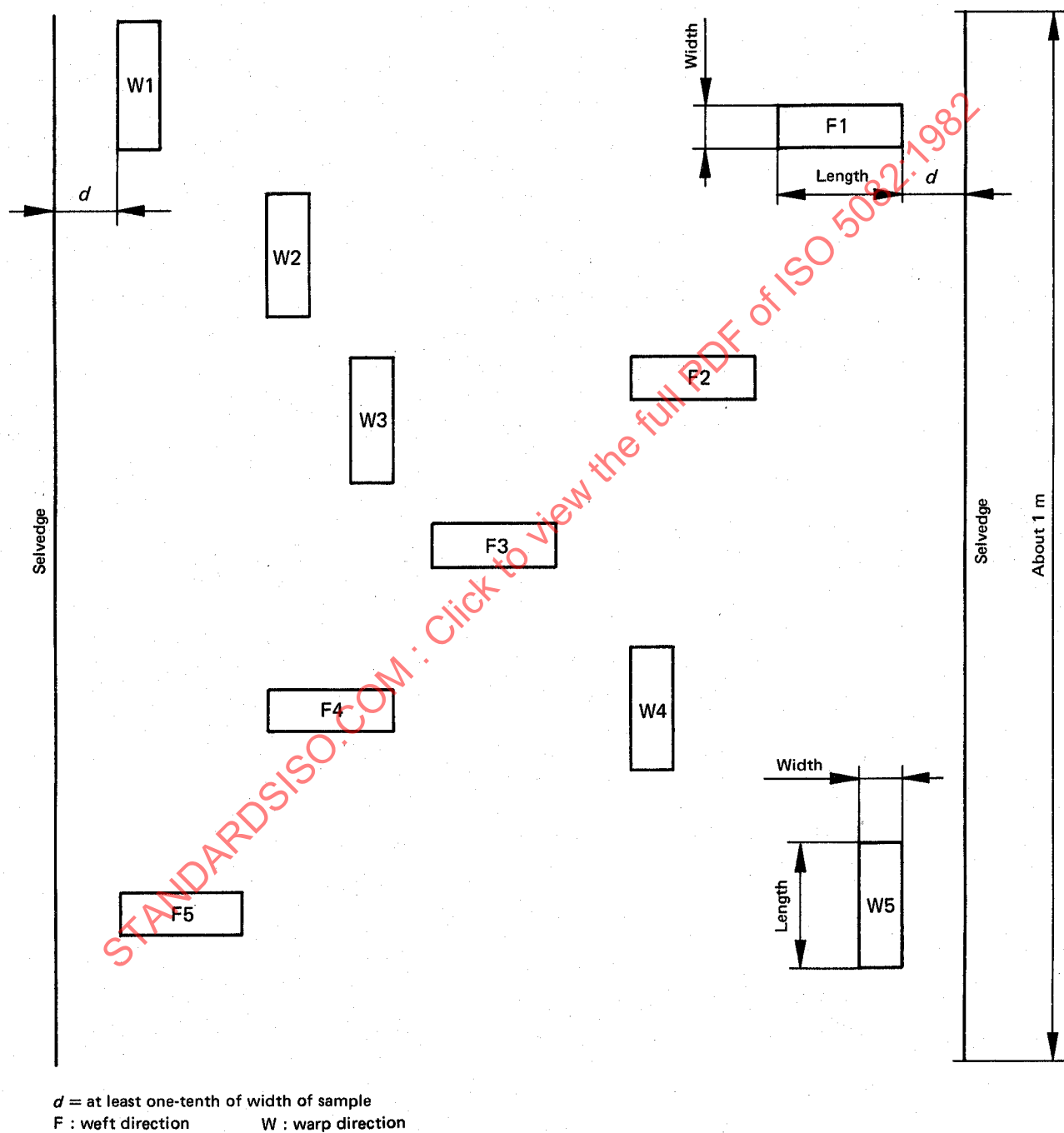
Figure — Example of cutting specimens
