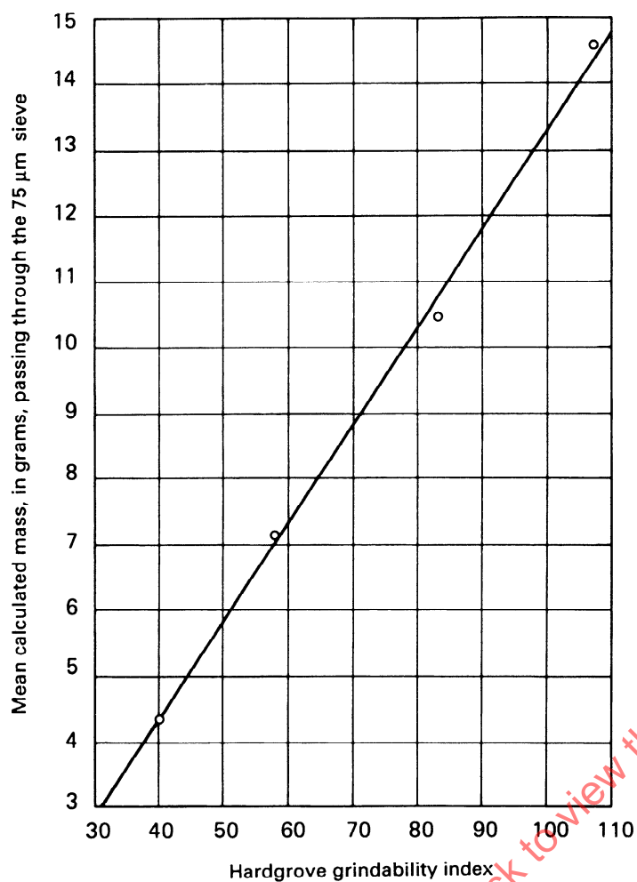
Figure A.1 — Specimen calibration chart
