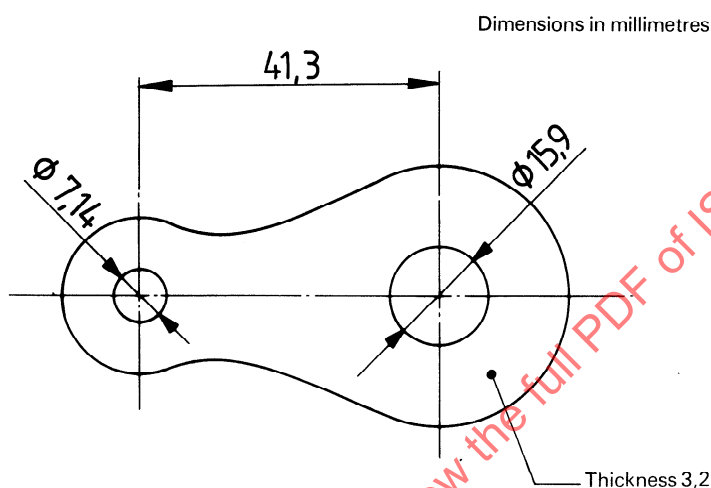
Figure A.1 — Ball support
