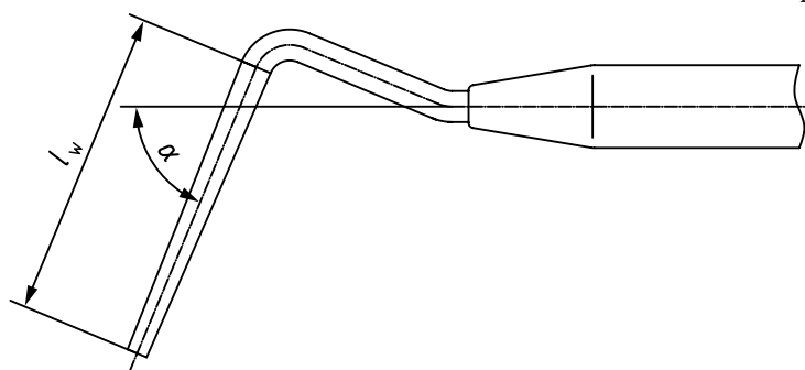
Figure 3 — Binangle compactor
