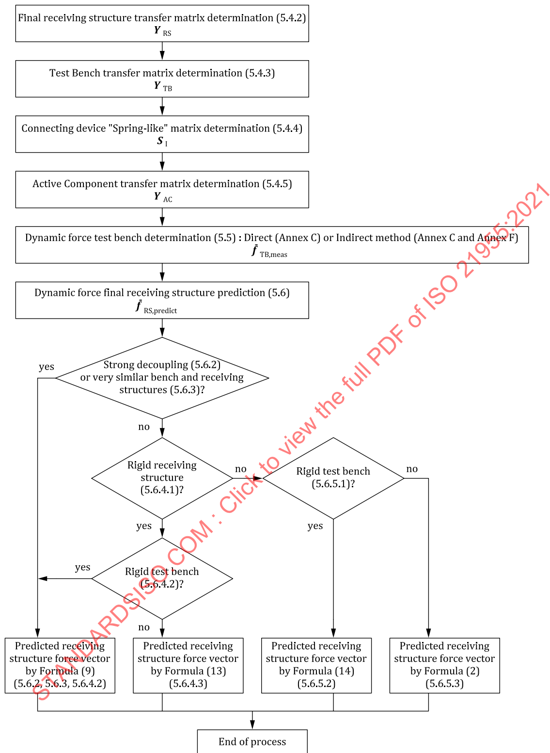
Figure 2 — Synoptic of the steps to determine predicted force
