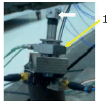
b) Middle fixation point (MFP)
