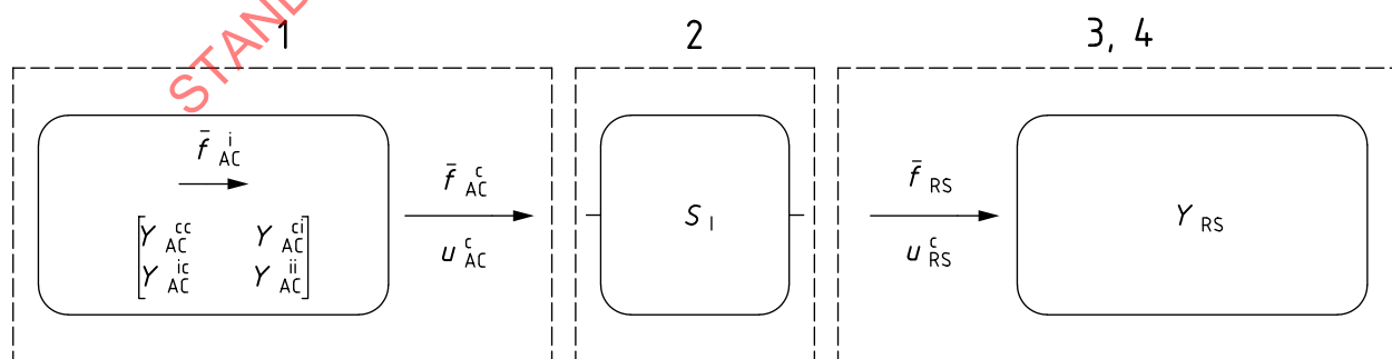
Figure A.1 — Detailed schematic of the structure assembly
