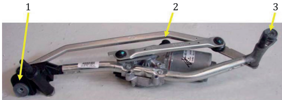
a) Active component: wiper system
