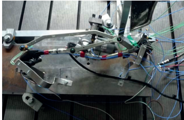
Figure E.10 — Active component mounted on the test bench clamped on the marble
