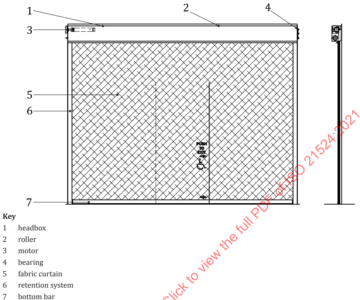
Figure 5 — Example of a typical active fire curtain with pass door(s)
