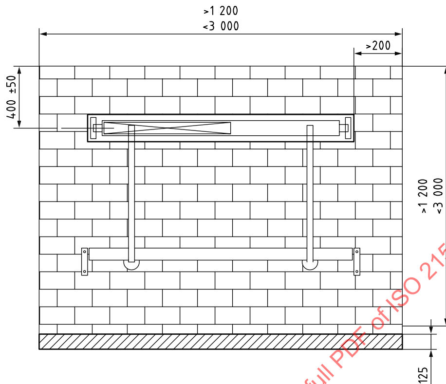
Figure F.4 — Elevation showing dimensions of a typical furnace in relation to specimen
