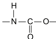
Figure C.1 — Urethane groups
