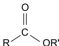
Figure C.2 — Ester bond
