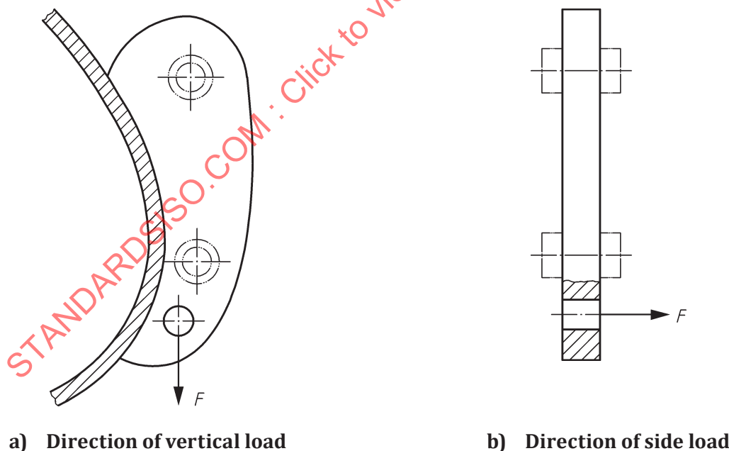
Figure C.2 — Load direction
