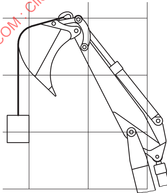
Figure C.1 — Sling guidance over back-wall of bucket
