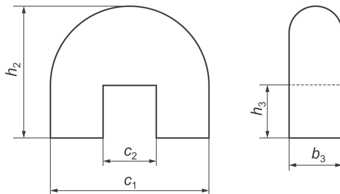
a) Pressure head used to apply cyclic load during interfacial tensile fatigue properties tests
