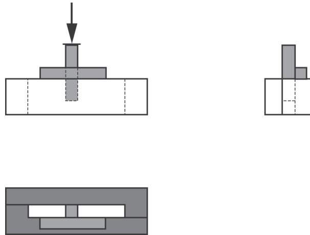
Figure 5 — Schematic diagram of the cross-bonded test piece and fixture for measuring the interfacial shear/shear fatigue properties
