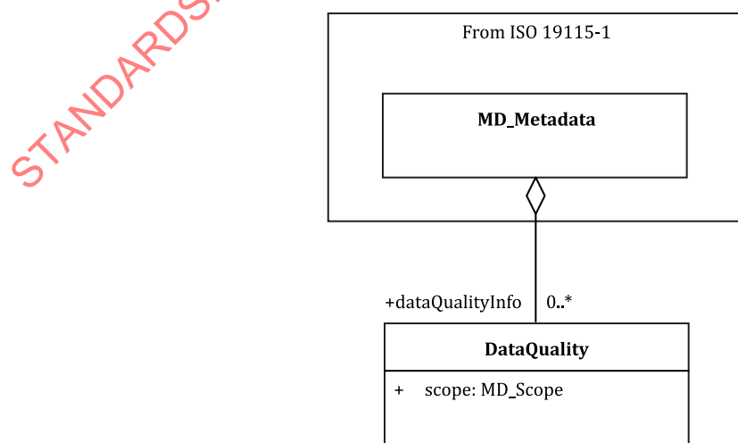
Figure B.2 — Data quality information
