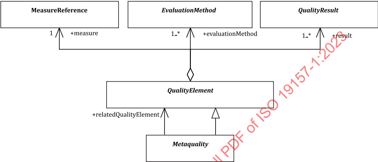
Figure 9 — Metaquality descriptors
