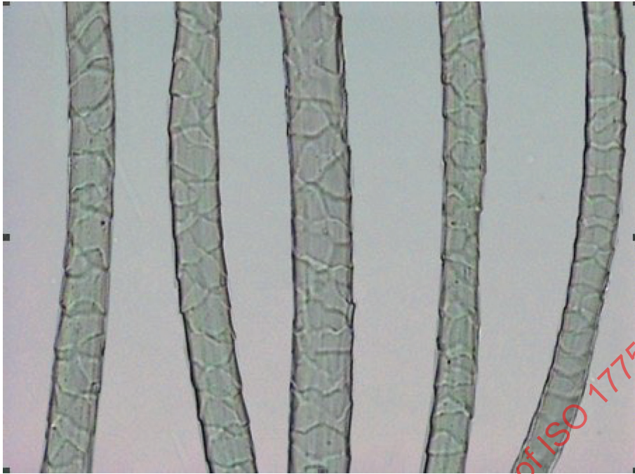
Figure C.31 — Irregular scale on unsmooth fibre surfaces
