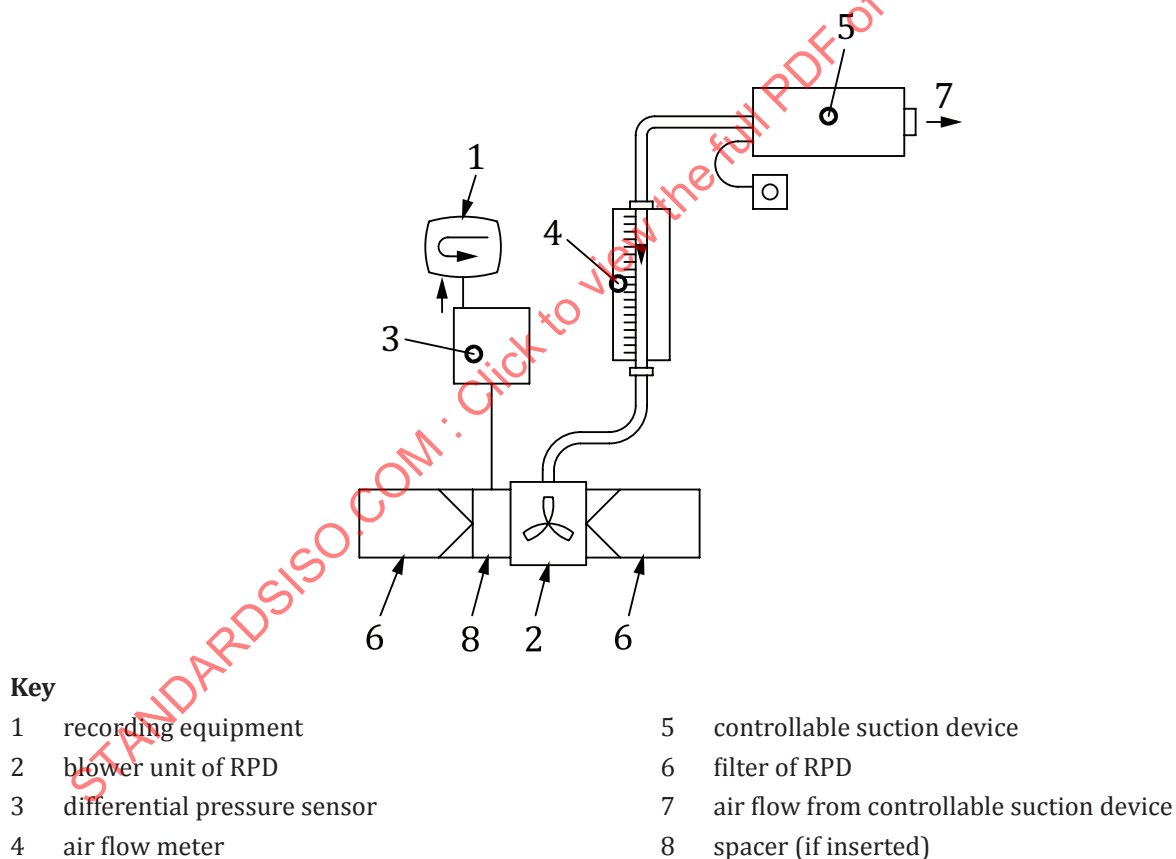
Figure 4 — Typical test arrangement for calibration
