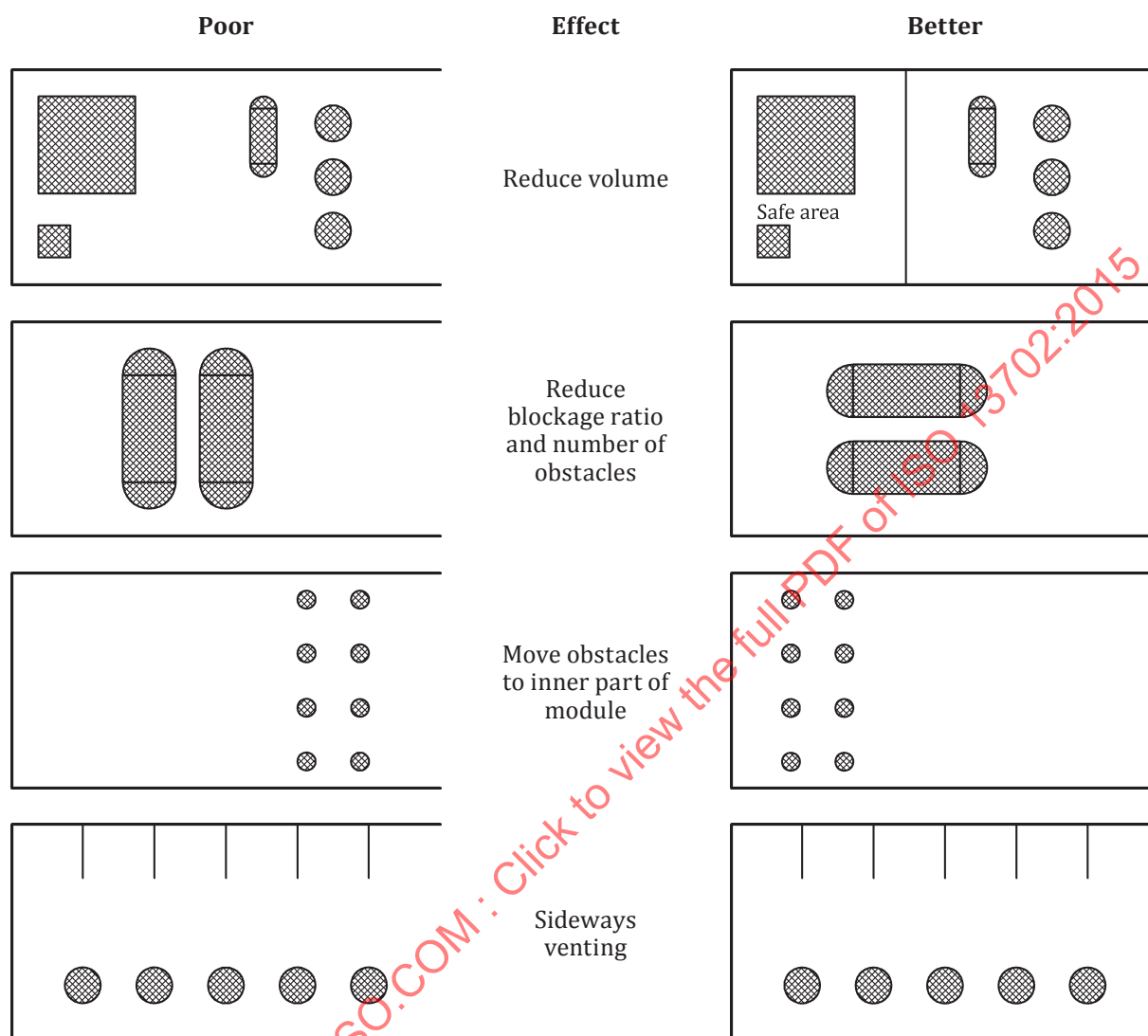
Figure B.1 — Effect of layout on explosion severity
