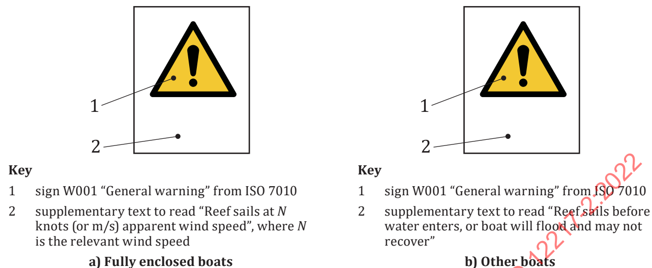
Figure 7 — Reefing safety signs
