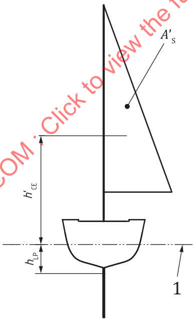
Figure 5 — Wind stiffness test
