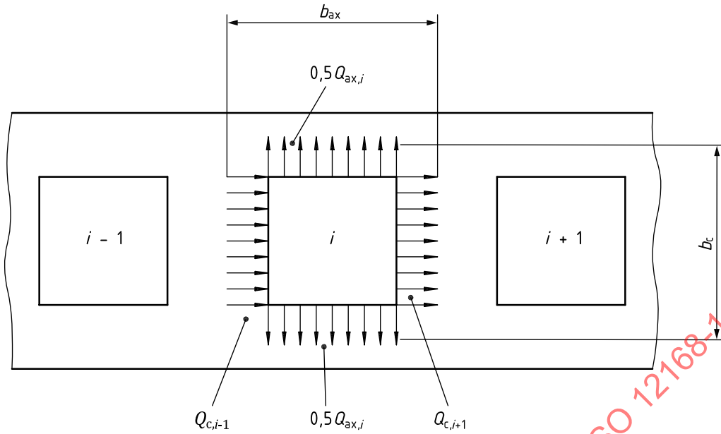
Figure A.4 — Volume flows for one recess
