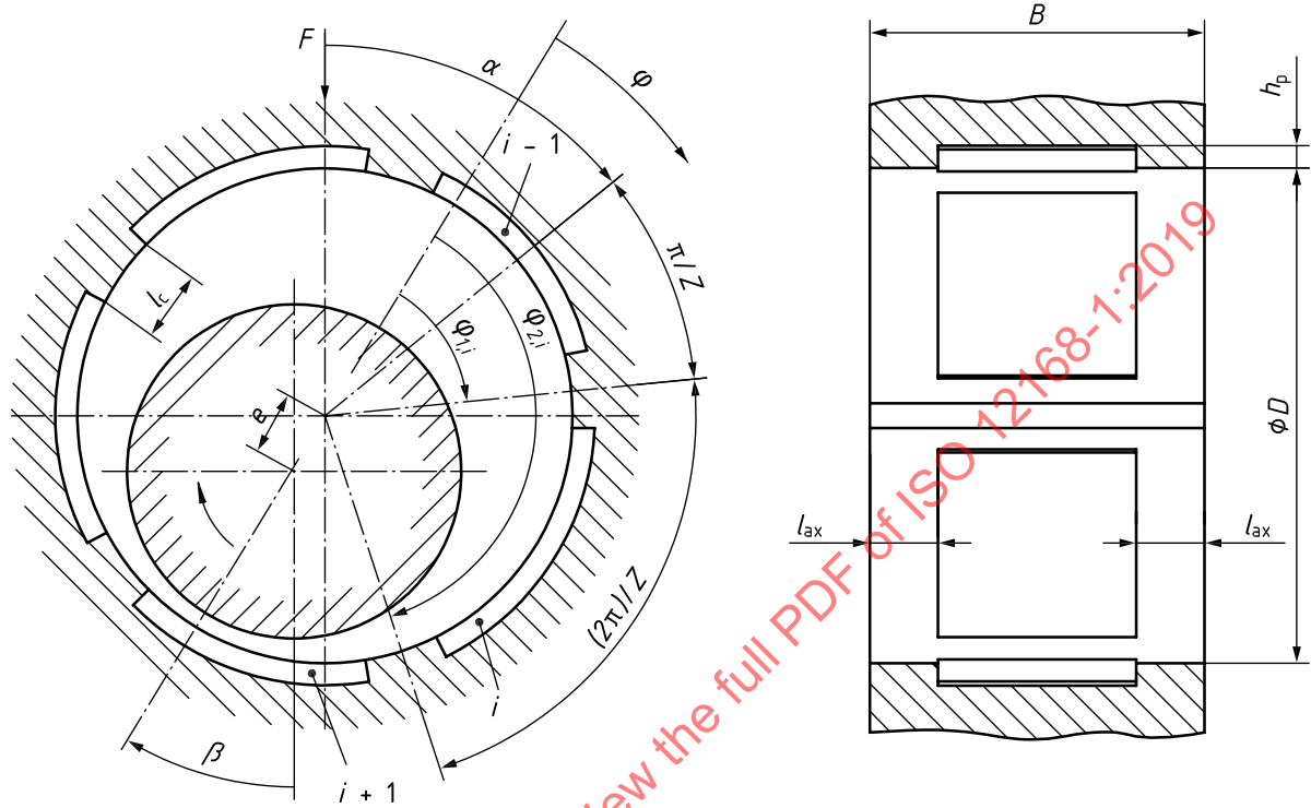
Figure A.3 — Bearing geometry
