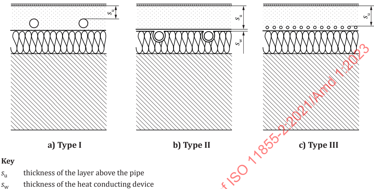
Figure A.1 — Definition of s_u for the different system types
